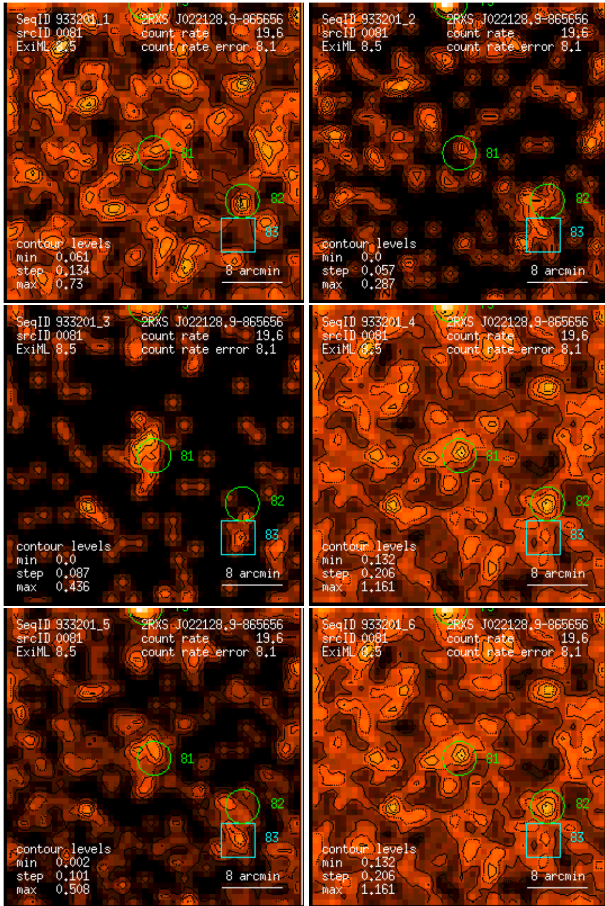
Figure 81: RASS 933201: detection 0081: band rate images, Gaussian filter: (1) PSPC channels 11 – 41, (2) 52 – 90, (3) 91 – 201, (4) 11 – 235, (5) 52 – 201, (6) 11 – 201. Broad band rates in counts/ks. Band rate contour levels in counts/ks/arcmin 2 .
