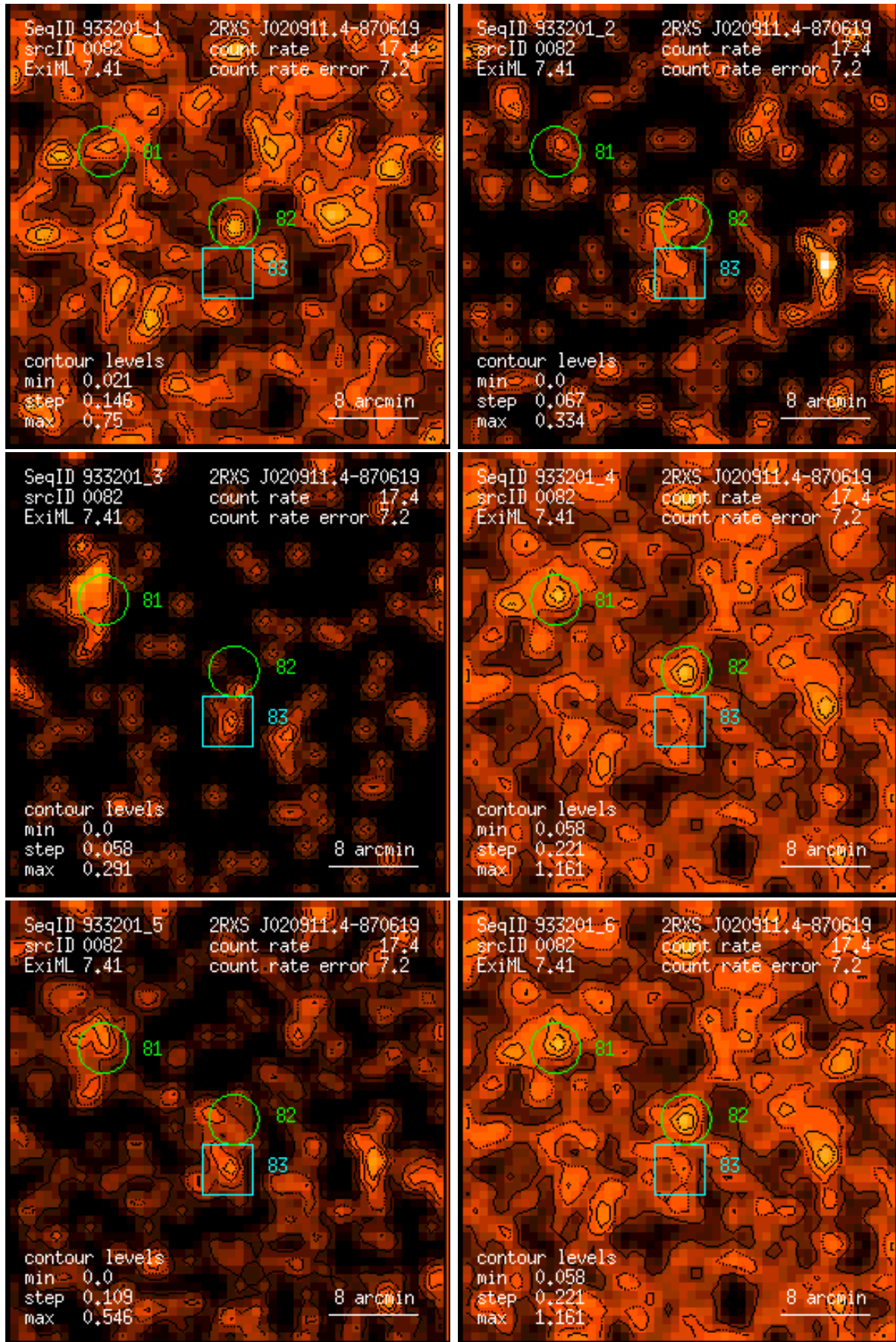
Figure 82: RASS 933201: detection 0082: band rate images, Gaussian filter: (1) PSPC channels 11 – 41, (2) 52 – 90, (3) 91 – 201, (4) 11 – 235, (5) 52 – 201, (6) 11 – 201. Broad band rates in counts/ks. Band rate contour levels in counts/ks/arcmin 2 .
