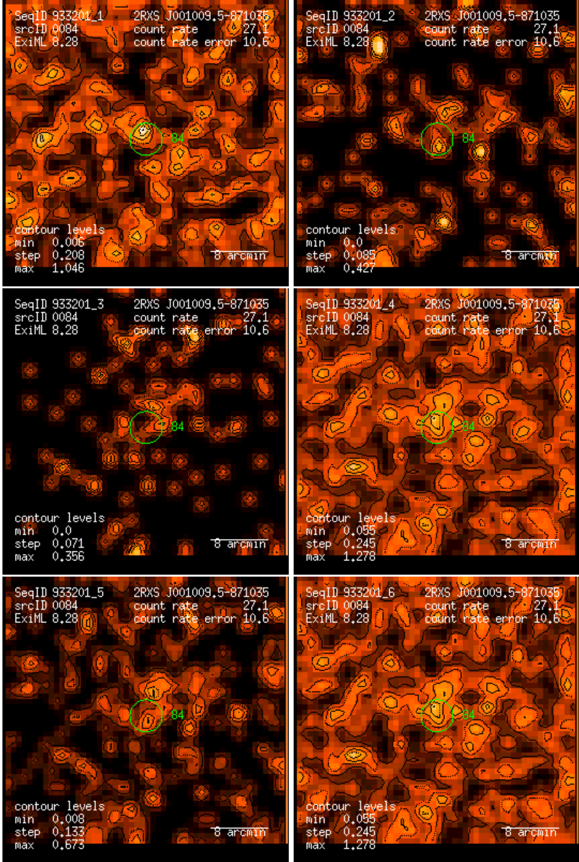
Figure 84: RASS 933201: detection 0084: band rate images, Gaussian filter: (1) PSPC channels 11 – 41, (2) 52 – 90, (3) 91 – 201, (4) 11 – 235, (5) 52 – 201, (6) 11 – 201. Broad band rates in counts/ks. Band rate contour levels in counts/ks/arcmin 2 .
