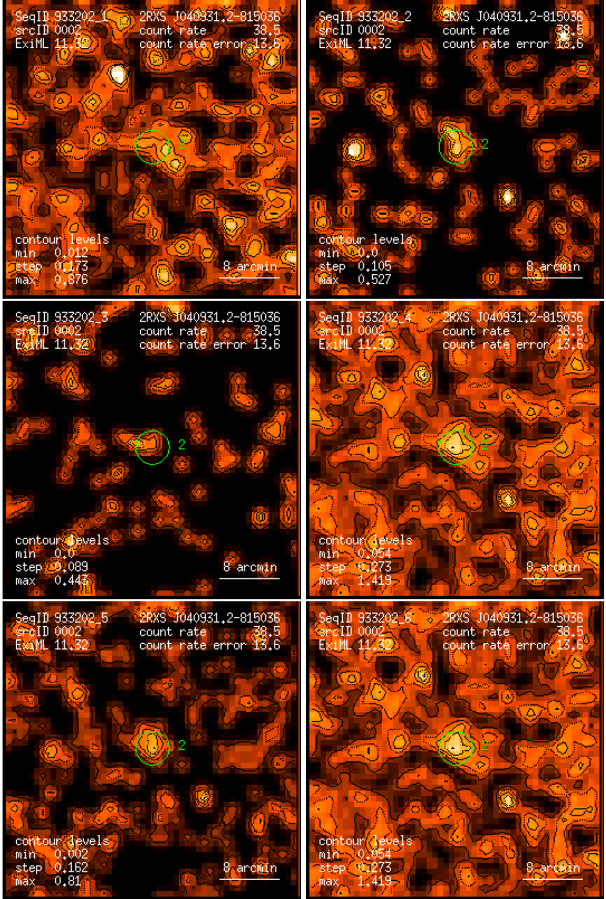
Figure 2: RASS 933202: detection 0002: band rate images, Gaussian filter: (1) PSPC channels 11 – 41, (2) 52 – 90, (3) 91 – 201, (4) 11 – 235, (5) 52 – 201, (6) 11 – 201. Broad band rates in counts/ks. Band rate contour levels in counts/ks/arcmin 2 .
