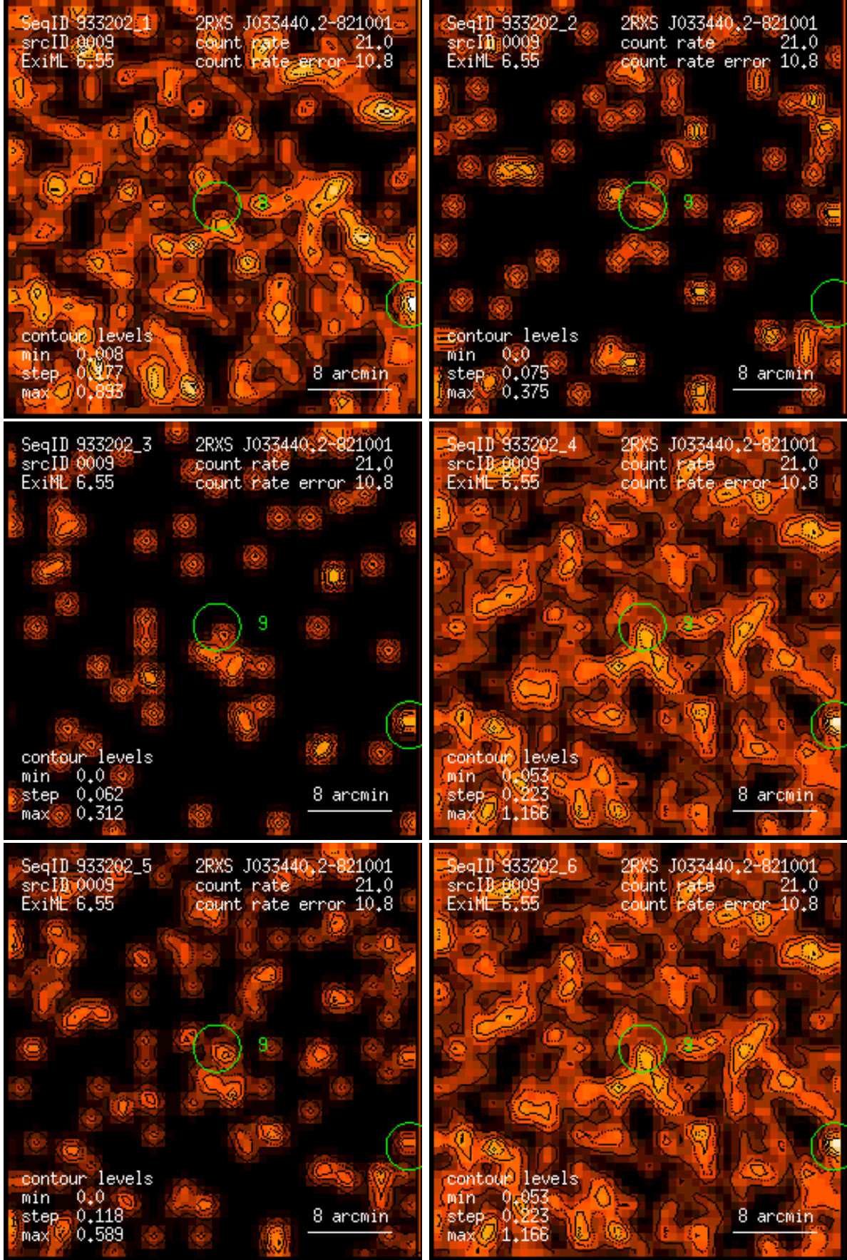
Figure 9: RASS 933202: detection 0009: band rate images, Gaussian filter: (1) PSPC channels 11 – 41, (2) 52 – 90, (3) 91 – 201, (4) 11 – 235, (5) 52 – 201, (6) 11 – 201. Broad band rates in counts/ks. Band rate contour levels in counts/ks/arcmin 2 .
