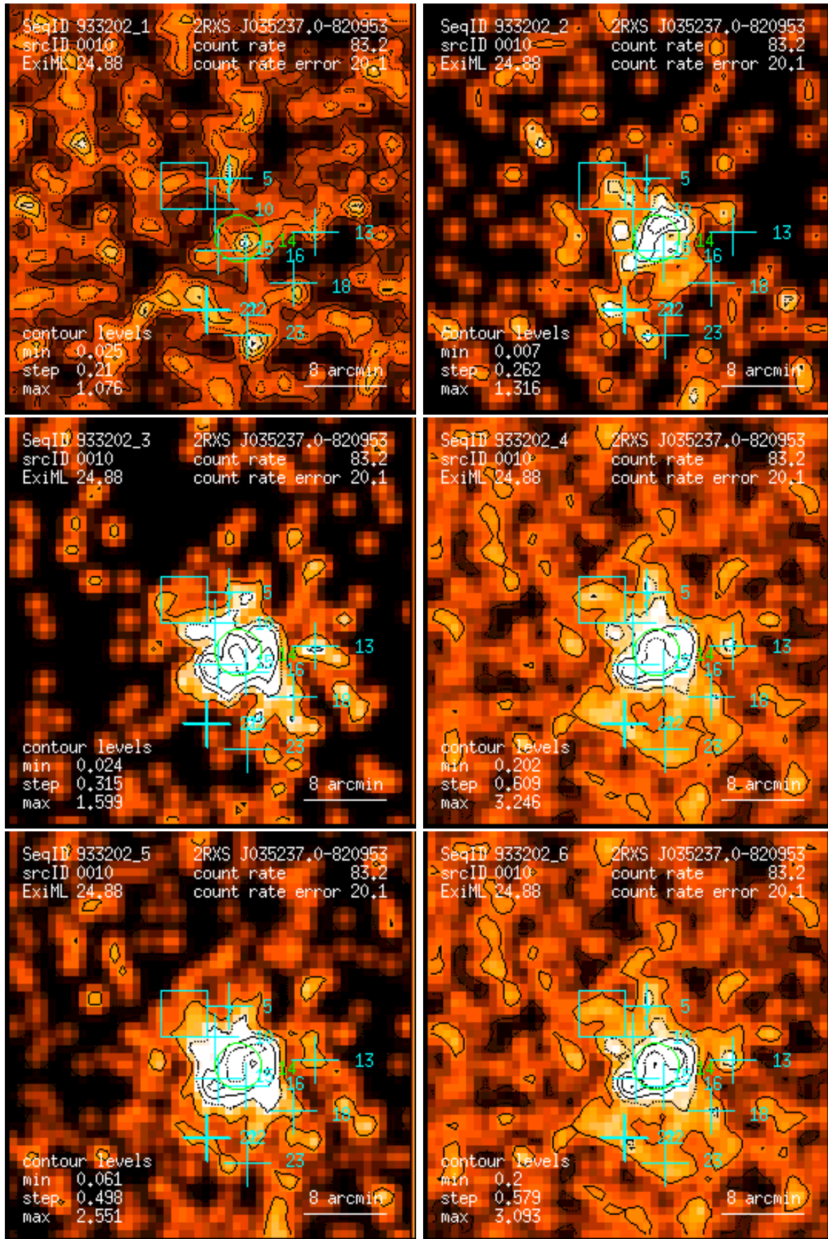
Figure 10: RASS 933202: detection 0010: band rate images, Gaussian filter: (1) PSPC channels 11 – 41, (2) 52 – 90, (3) 91 – 201, (4) 11 – 235, (5) 52 – 201, (6) 11 – 201. Broad band rates in counts/ks. Band rate contour levels in counts/ks/arcmin 2 .
