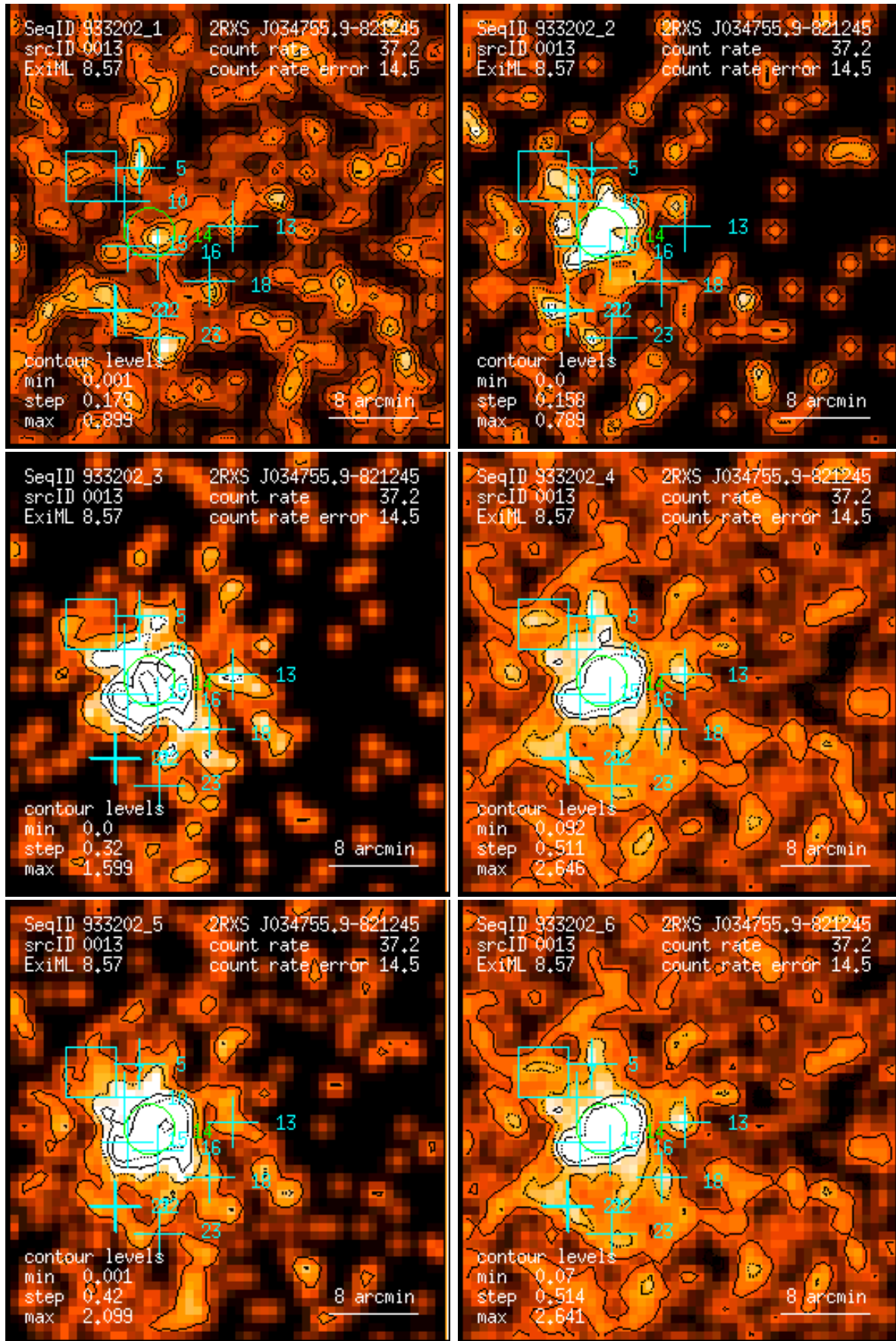
Figure 13: RASS 933202: detection 0013: band rate images, Gaussian filter: (1) PSPC channels 11 – 41, (2) 52 – 90, (3) 91 – 201, (4) 11 – 235, (5) 52 – 201, (6) 11 – 201. Broad band rates in counts/ks. Band rate contour levels in counts/ks/arcmin 2 .
