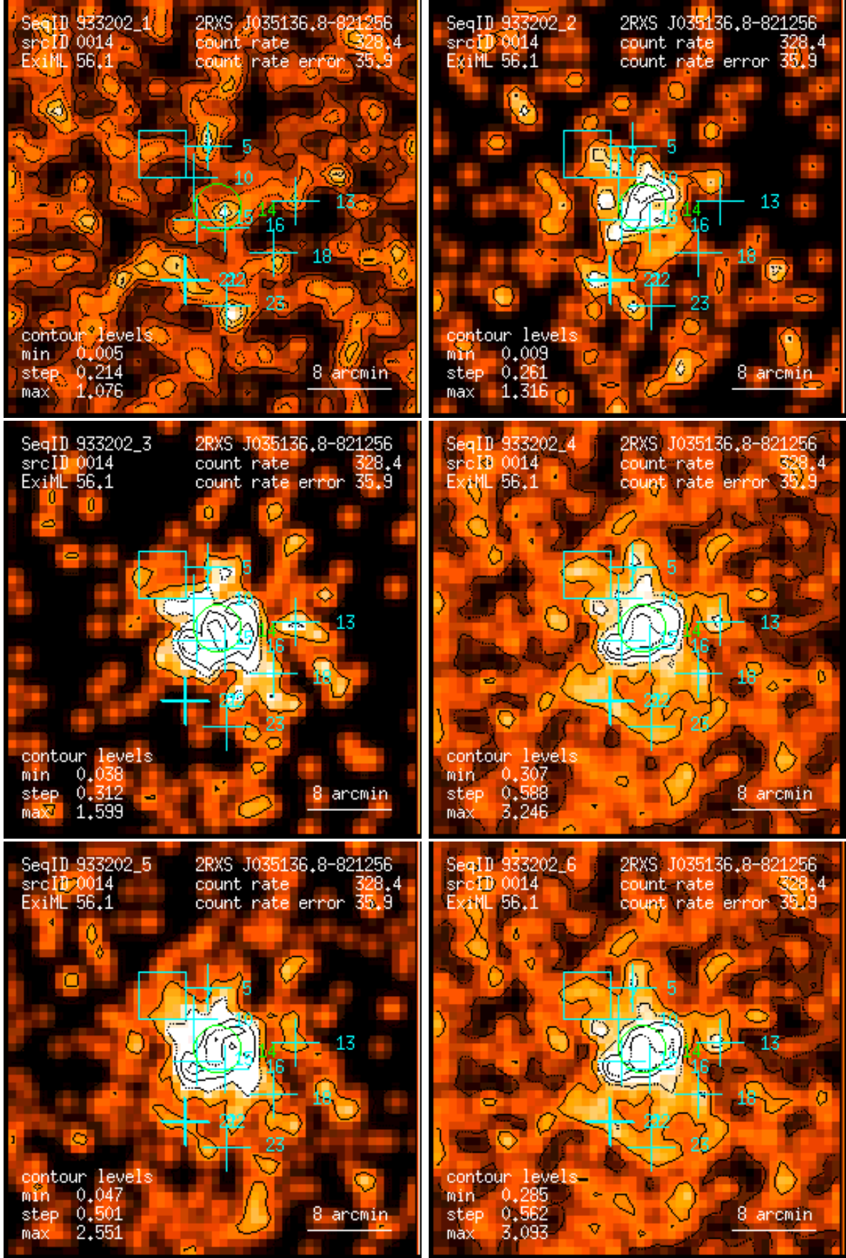
Figure 14: RASS 933202: detection 0014: band rate images, Gaussian filter: (1) PSPC channels 11 – 41, (2) 52 – 90, (3) 91 – 201, (4) 11 – 235, (5) 52 – 201, (6) 11 – 201. Broad band rates in counts/ks. Band rate contour levels in counts/ks/arcmin 2 .
