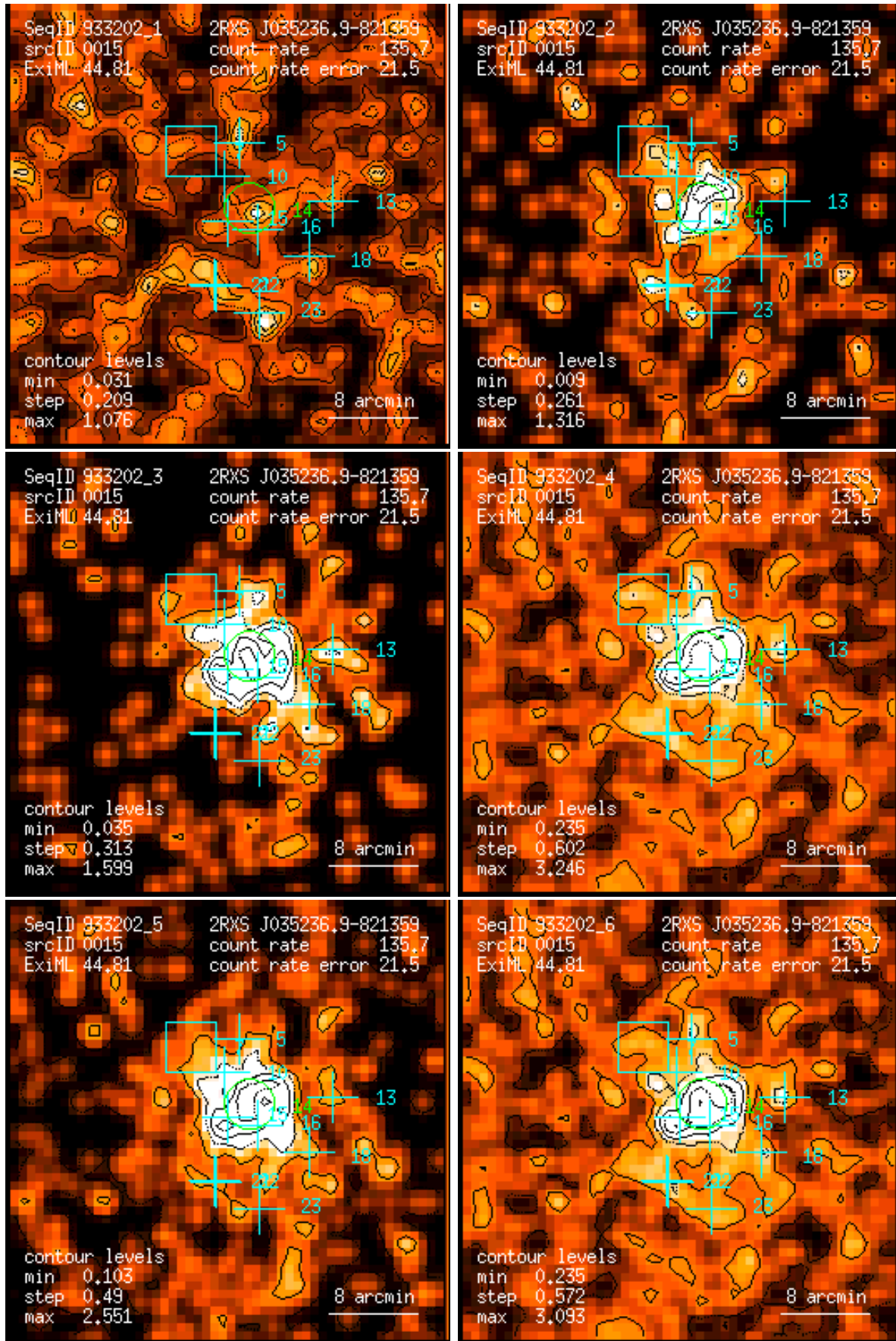
Figure 15: RASS 933202: detection 0015: band rate images, Gaussian filter: (1) PSPC channels 11 – 41, (2) 52 – 90, (3) 91 – 201, (4) 11 – 235, (5) 52 – 201, (6) 11 – 201. Broad band rates in counts/ks. Band rate contour levels in counts/ks/arcmin 2 .
