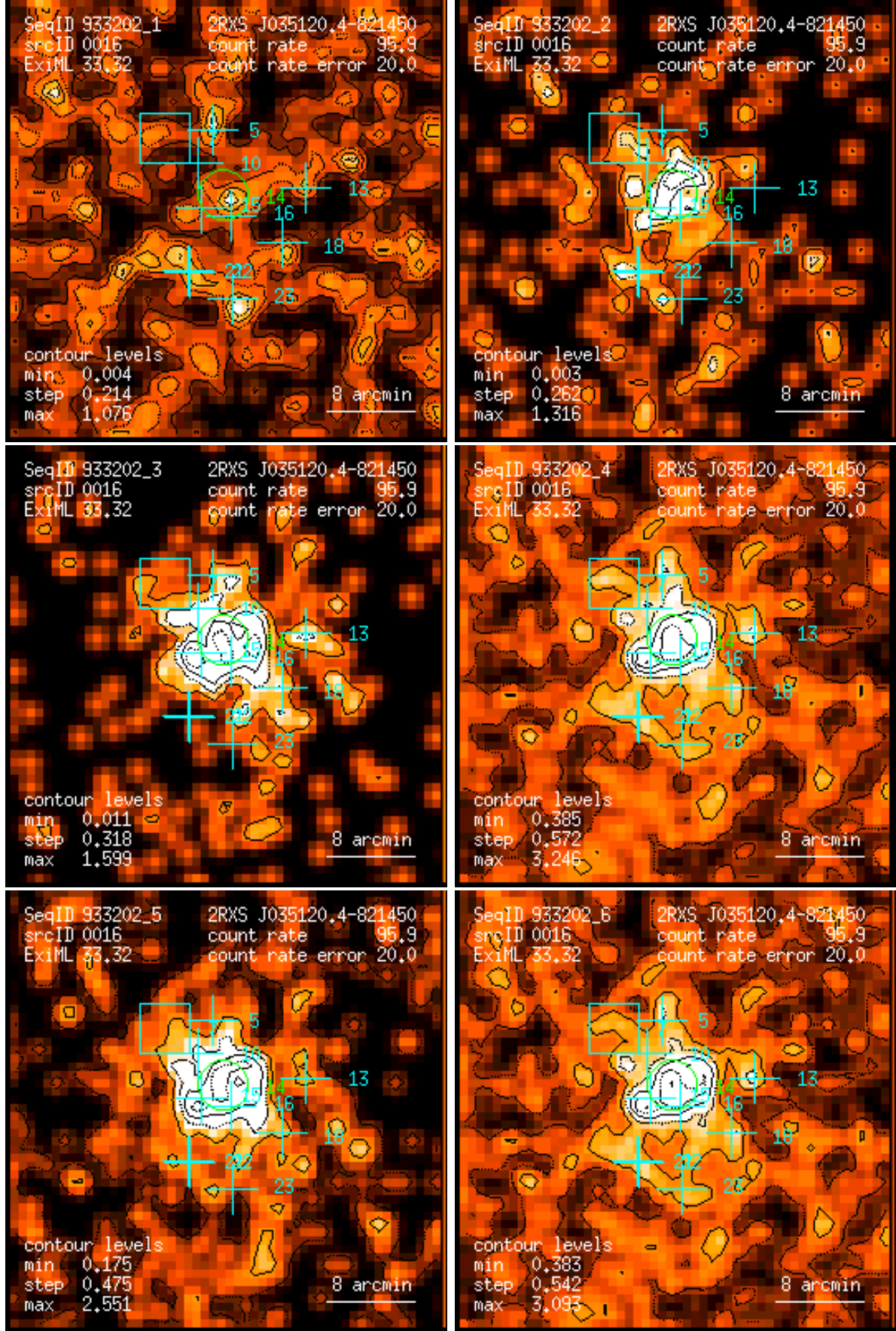
Figure 16: RASS 933202: detection 0016: band rate images, Gaussian filter: (1) PSPC channels 11 – 41, (2) 52 – 90, (3) 91 – 201, (4) 11 – 235, (5) 52 – 201, (6) 11 – 201. Broad band rates in counts/ks. Band rate contour levels in counts/ks/arcmin 2 .
