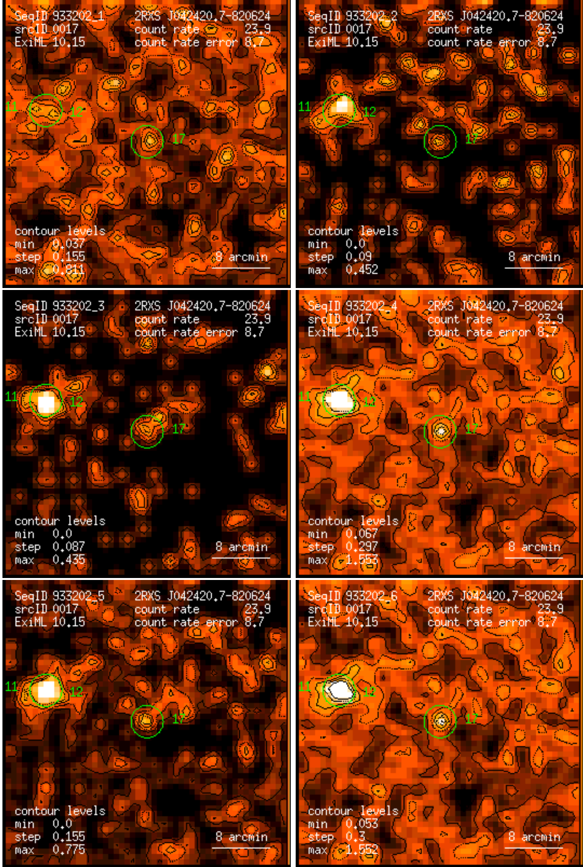
Figure 17: RASS 933202: detection 0017: band rate images, Gaussian filter: (1) PSPC channels 11 – 41, (2) 52 – 90, (3) 91 – 201, (4) 11 – 235, (5) 52 – 201, (6) 11 – 201. Broad band rates in counts/ks. Band rate contour levels in counts/ks/arcmin 2 .
