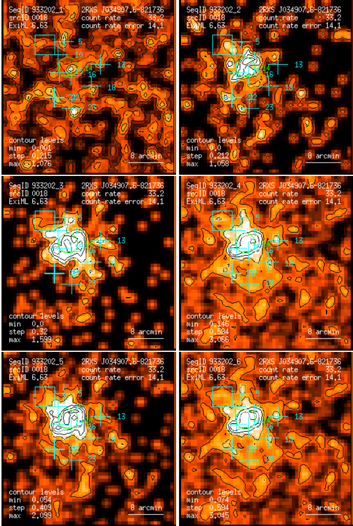
Figure 18: RASS 933202: detection 0018: band rate images, Gaussian filter: (1) PSPC channels 11 – 41, (2) 52 – 90, (3) 91 – 201, (4) 11 – 235, (5) 52 – 201, (6) 11 – 201. Broad band rates in counts/ks. Band rate contour levels in counts/ks/arcmin 2 .
