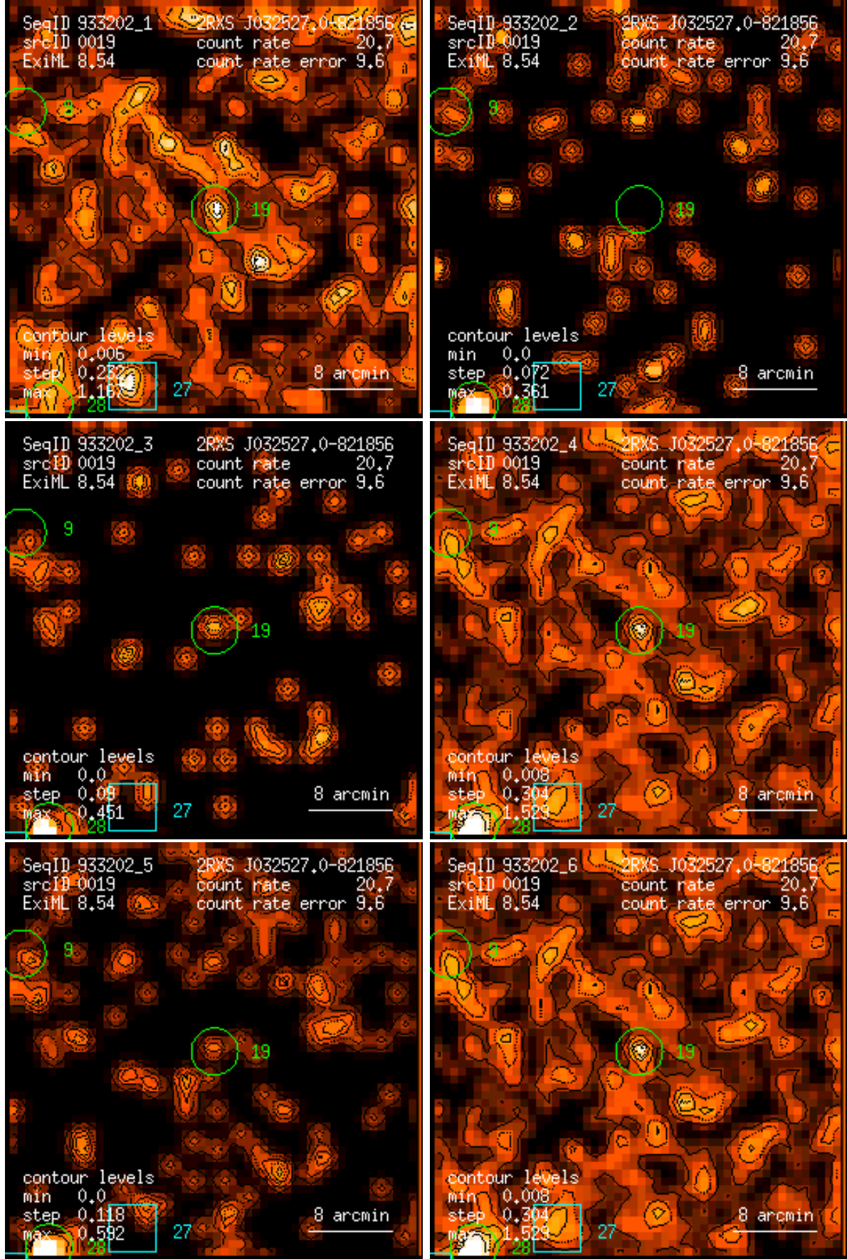
Figure 19: RASS 933202: detection 0019: band rate images, Gaussian filter: (1) PSPC channels 11 – 41, (2) 52 – 90, (3) 91 – 201, (4) 11 – 235, (5) 52 – 201, (6) 11 – 201. Broad band rates in counts/ks. Band rate contour levels in counts/ks/arcmin 2 .
