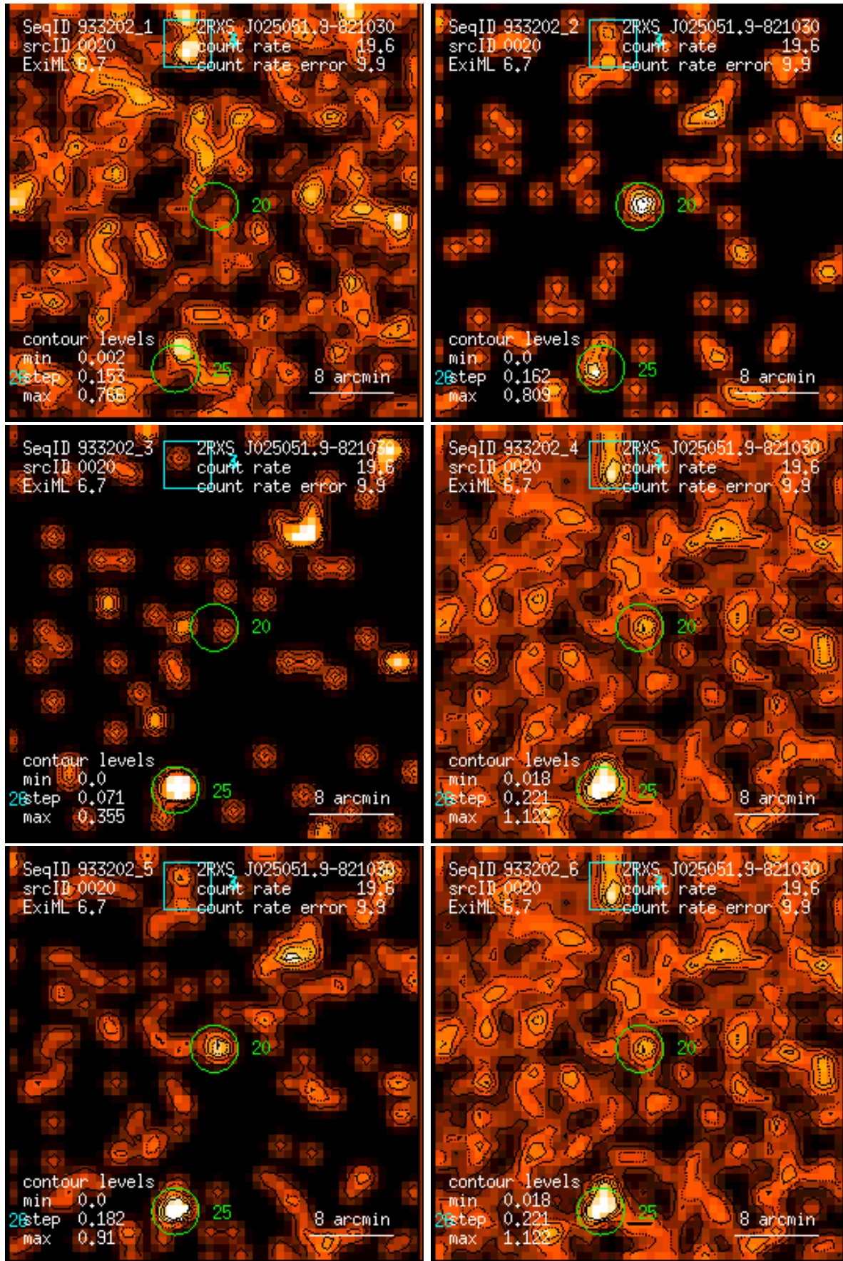
Figure 20: RASS 933202: detection 0020: band rate images, Gaussian filter: (1) PSPC channels 11 – 41, (2) 52 – 90, (3) 91 – 201, (4) 11 – 235, (5) 52 – 201, (6) 11 – 201. Broad band rates in counts/ks. Band rate contour levels in counts/ks/arcmin 2 .
