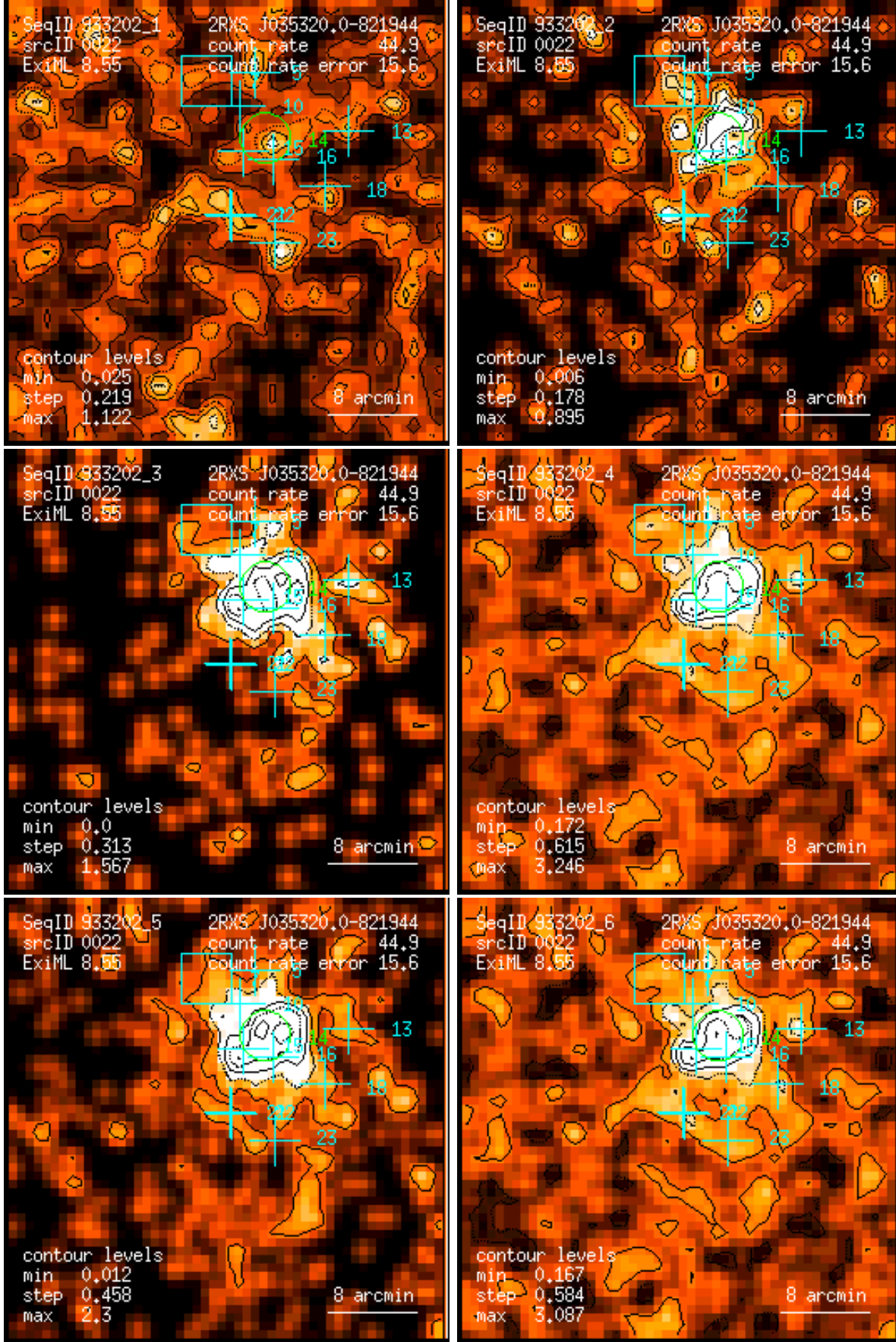
Figure 22: RASS 933202: detection 0022: band rate images, Gaussian filter: (1) PSPC channels 11 – 41, (2) 52 – 90, (3) 91 – 201, (4) 11 – 235, (5) 52 – 201, (6) 11 – 201. Broad band rates in counts/ks. Band rate contour levels in counts/ks/arcmin 2 .
