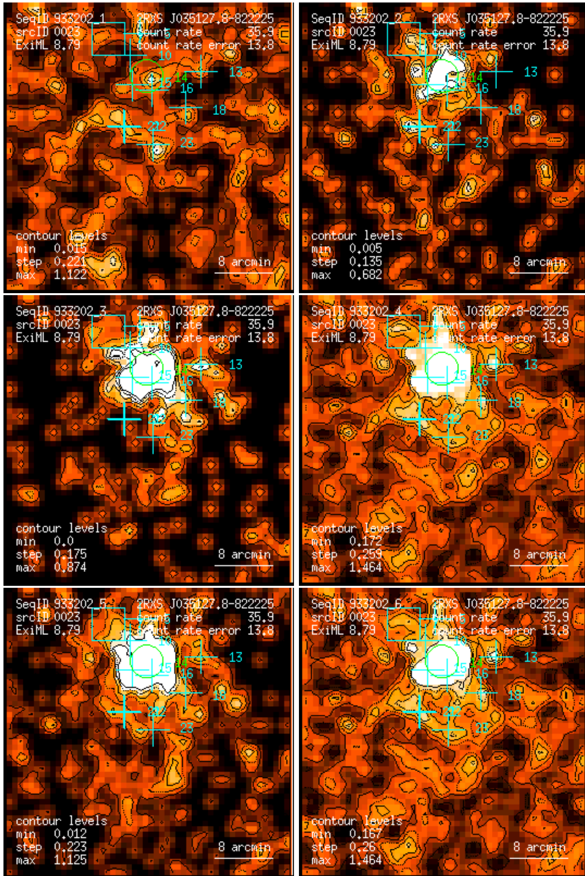
Figure 23: RASS 933202: detection 0023: band rate images, Gaussian filter: (1) PSPC channels 11 – 41, (2) 52 – 90, (3) 91 – 201, (4) 11 – 235, (5) 52 – 201, (6) 11 – 201. Broad band rates in counts/ks. Band rate contour levels in counts/ks/arcmin 2 .
