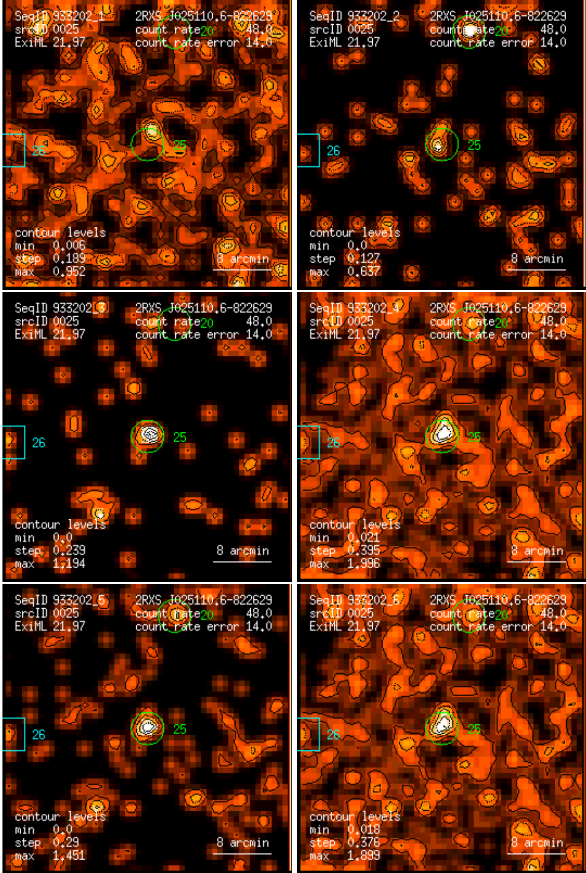
Figure 25: RASS 933202: detection 0025: band rate images, Gaussian filter: (1) PSPC channels 11 – 41, (2) 52 – 90, (3) 91 – 201, (4) 11 – 235, (5) 52 – 201, (6) 11 – 201. Broad band rates in counts/ks. Band rate contour levels in counts/ks/arcmin 2 .
