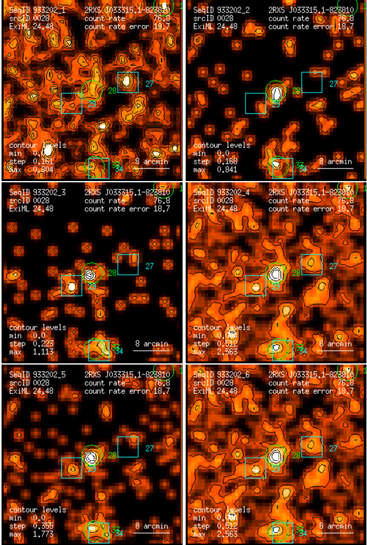
Figure 28: RASS 933202: detection 0028: band rate images, Gaussian filter: (1) PSPC channels 11 – 41, (2) 52 – 90, (3) 91 – 201, (4) 11 – 235, (5) 52 – 201, (6) 11 – 201. Broad band rates in counts/ks. Band rate contour levels in counts/ks/arcmin 2 .
