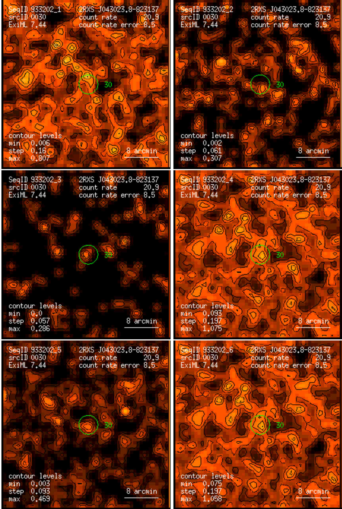
Figure 30: RASS 933202: detection 0030: band rate images, Gaussian filter: (1) PSPC channels 11 – 41, (2) 52 – 90, (3) 91 – 201, (4) 11 – 235, (5) 52 – 201, (6) 11 – 201. Broad band rates in counts/ks. Band rate contour levels in counts/ks/arcmin 2 .
