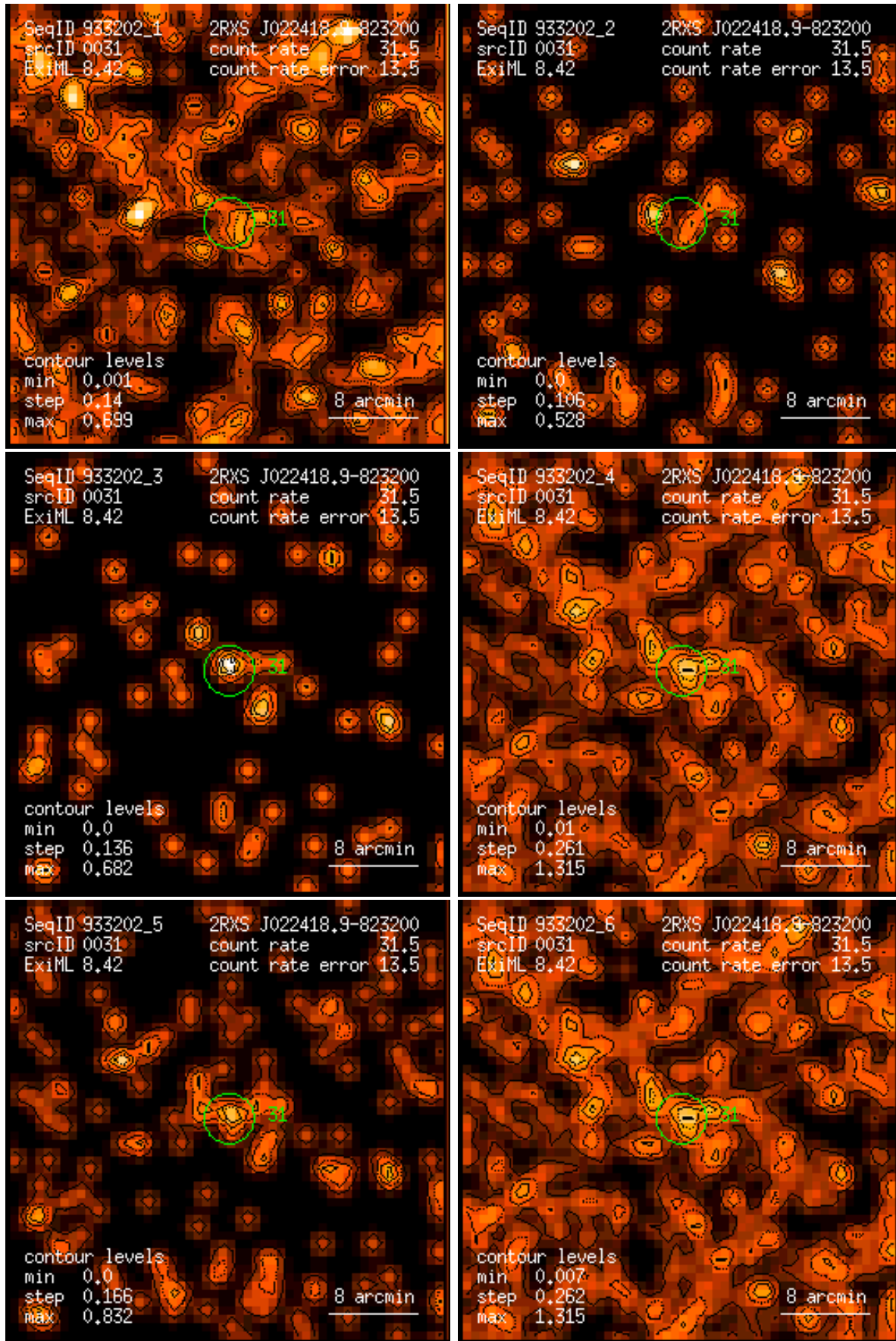
Figure 31: RASS 933202: detection 0031: band rate images, Gaussian filter: (1) PSPC channels 11 – 41, (2) 52 – 90, (3) 91 – 201, (4) 11 – 235, (5) 52 – 201, (6) 11 – 201. Broad band rates in counts/ks. Band rate contour levels in counts/ks/arcmin 2 .
