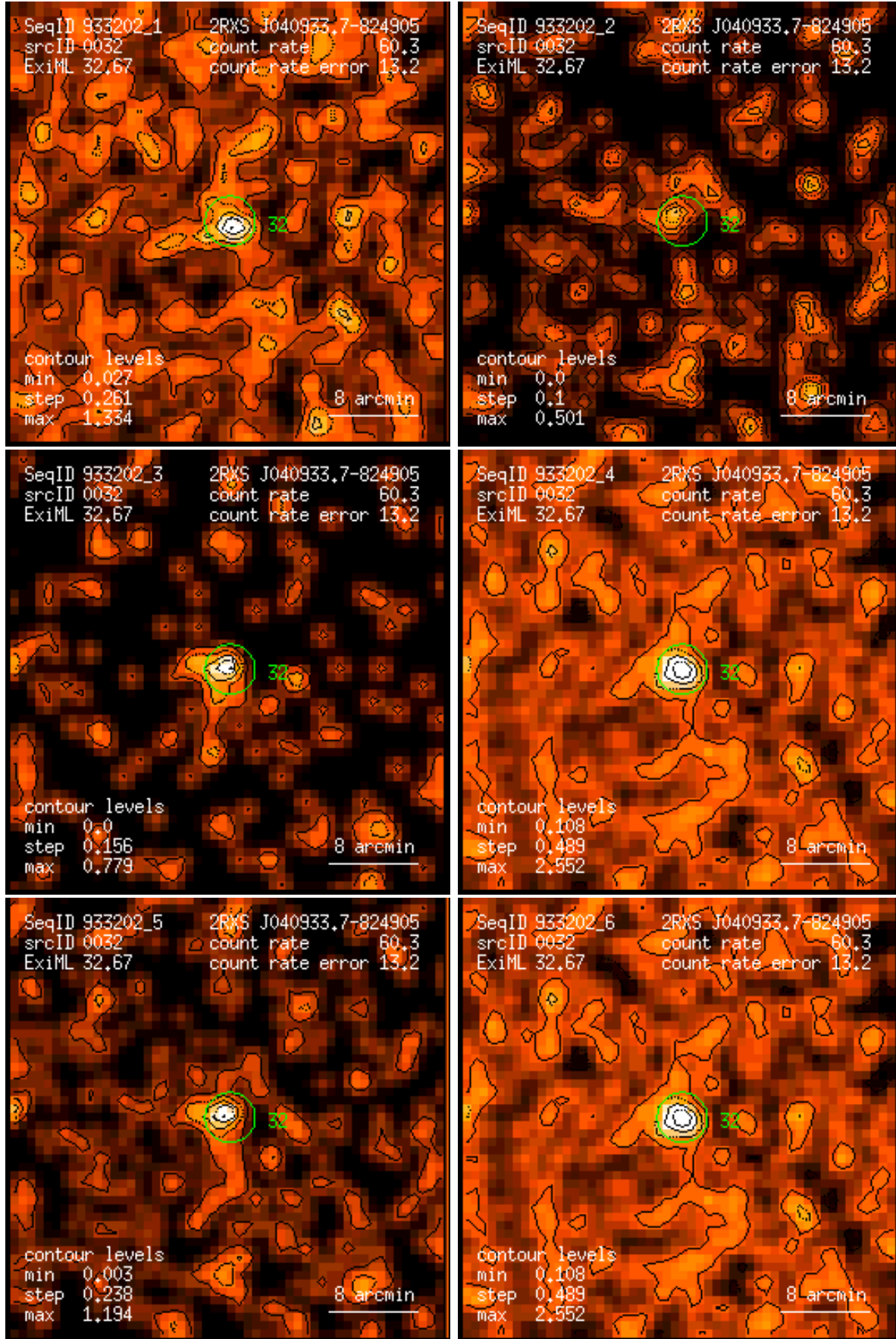
Figure 32: RASS 933202: detection 0032: band rate images, Gaussian filter: (1) PSPC channels 11 – 41, (2) 52 – 90, (3) 91 – 201, (4) 11 – 235, (5) 52 – 201, (6) 11 – 201. Broad band rates in counts/ks. Band rate contour levels in counts/ks/arcmin 2 .
