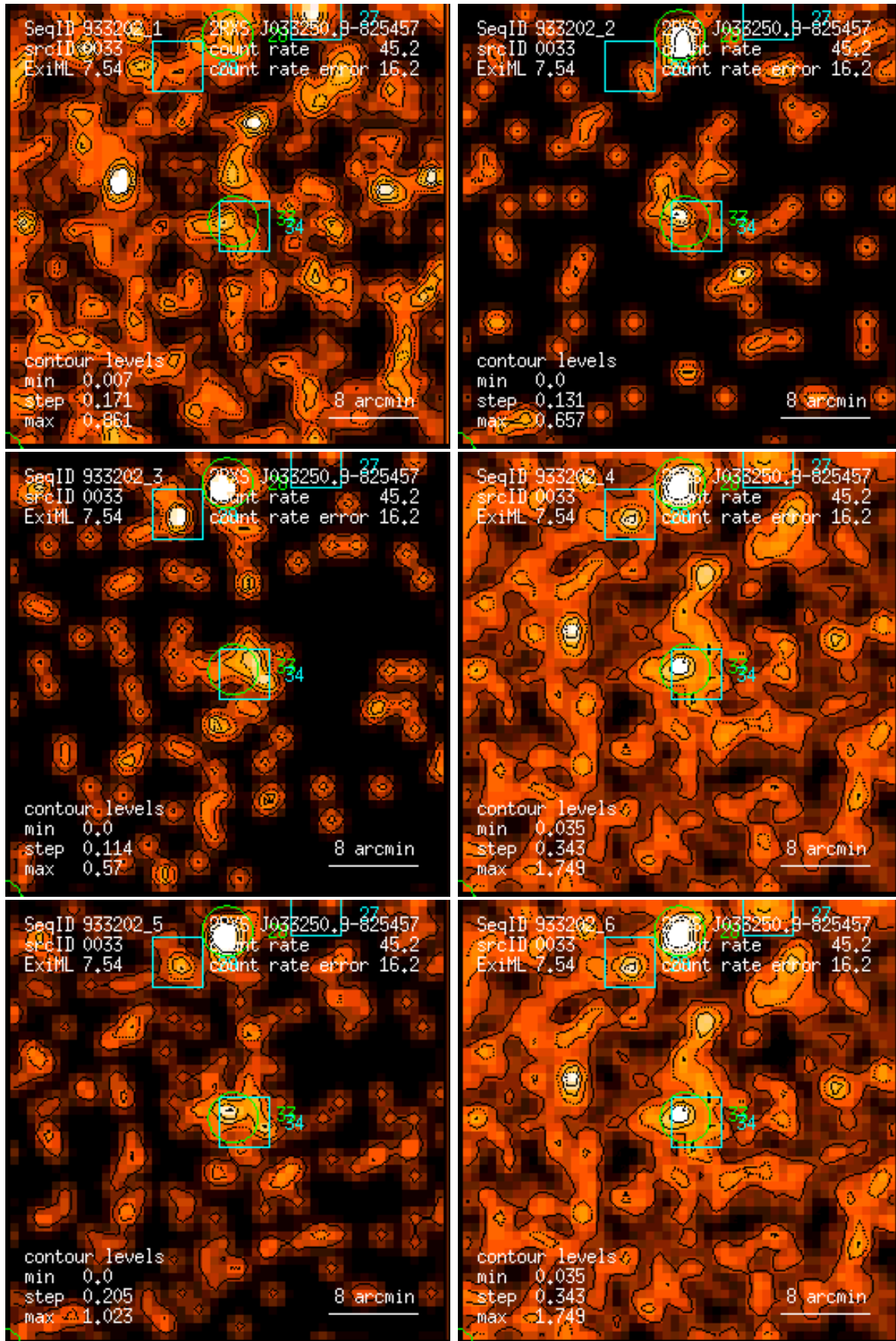
Figure 33: RASS 933202: detection 0033: band rate images, Gaussian filter: (1) PSPC channels 11 – 41, (2) 52 – 90, (3) 91 – 201, (4) 11 – 235, (5) 52 – 201, (6) 11 – 201. Broad band rates in counts/ks. Band rate contour levels in counts/ks/arcmin 2 .
