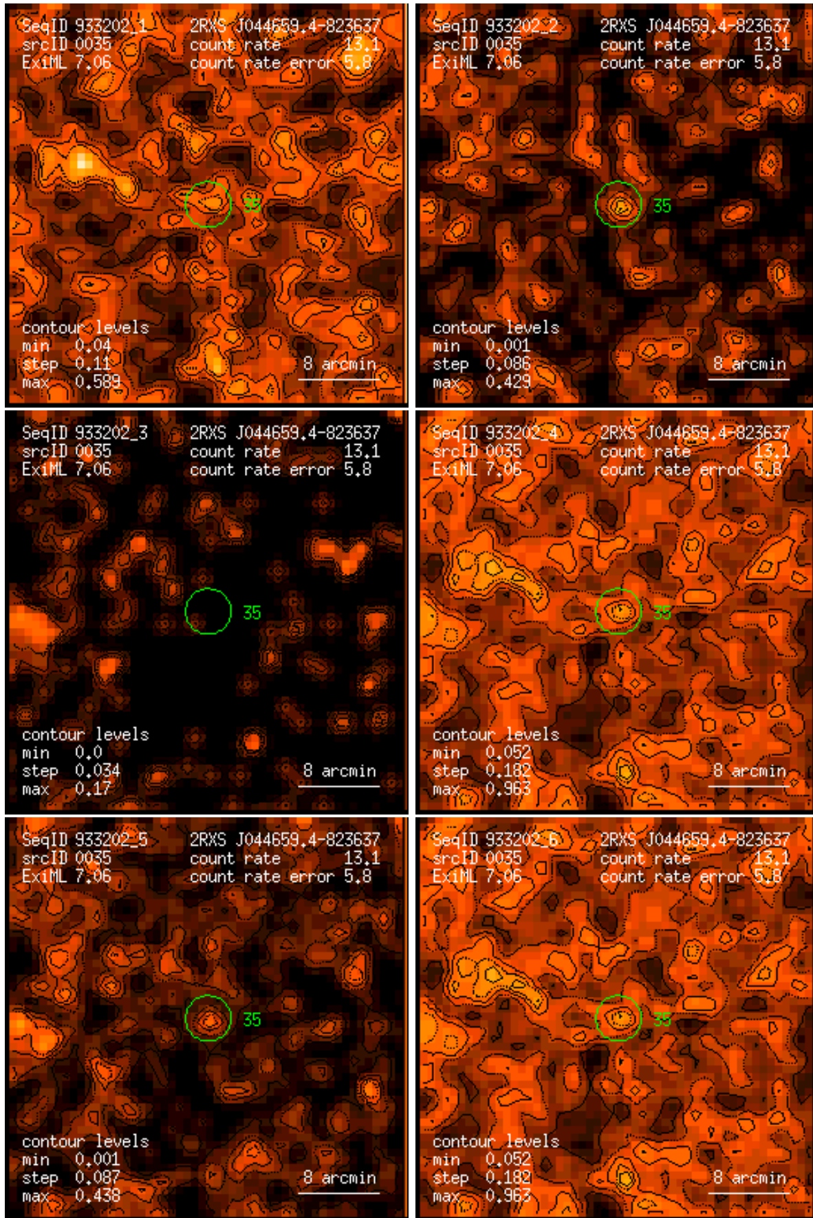
Figure 35: RASS 933202: detection 0035: band rate images, Gaussian filter: (1) PSPC channels 11 – 41, (2) 52 – 90, (3) 91 – 201, (4) 11 – 235, (5) 52 – 201, (6) 11 – 201. Broad band rates in counts/ks. Band rate contour levels in counts/ks/arcmin 2 .
