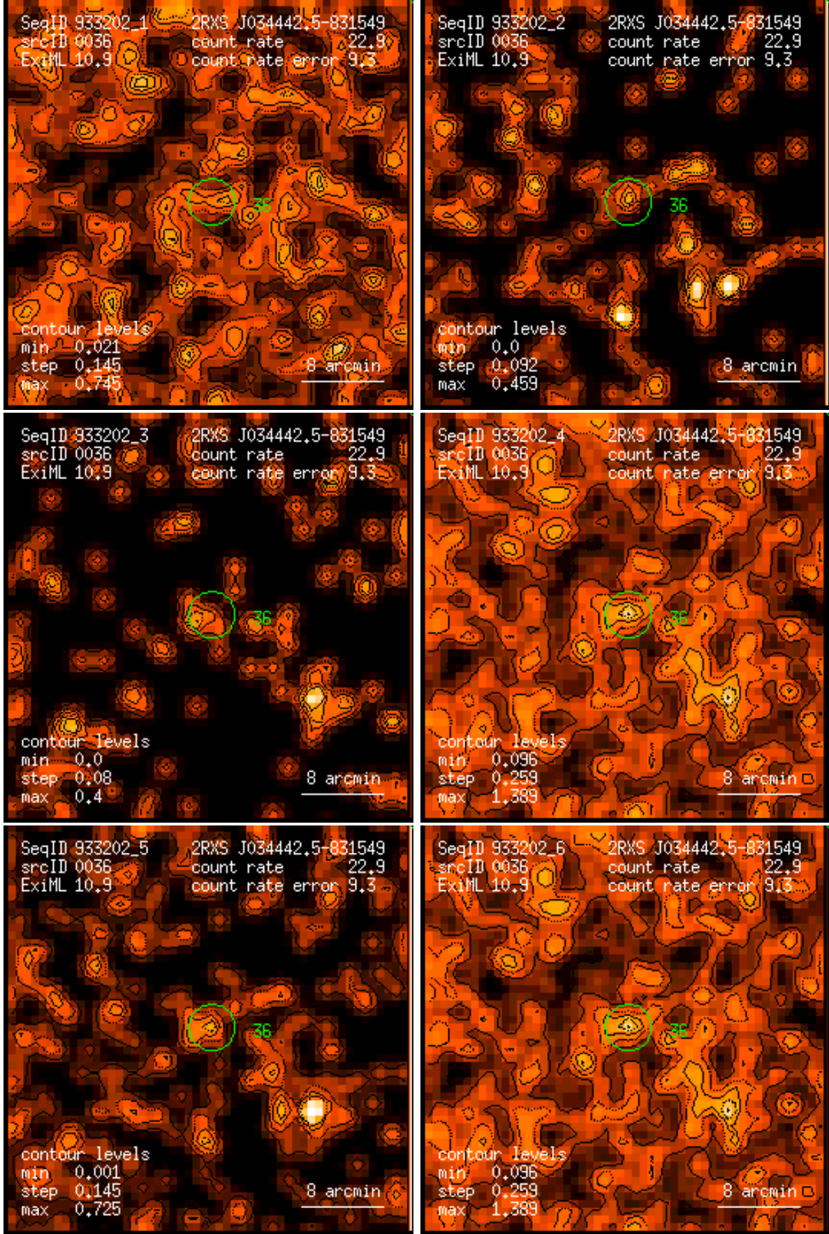
Figure 36: RASS 933202: detection 0036: band rate images, Gaussian filter: (1) PSPC channels 11 – 41, (2) 52 – 90, (3) 91 – 201, (4) 11 – 235, (5) 52 – 201, (6) 11 – 201. Broad band rates in counts/ks. Band rate contour levels in counts/ks/arcmin 2 .
