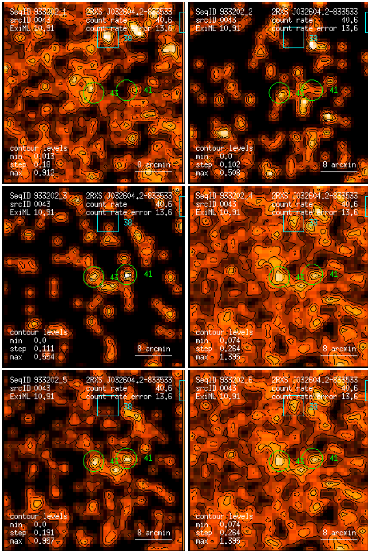
Figure 43: RASS 933202: detection 0043: band rate images, Gaussian filter: (1) PSPC channels 11 – 41, (2) 52 – 90, (3) 91 – 201, (4) 11 – 235, (5) 52 – 201, (6) 11 – 201. Broad band rates in counts/ks. Band rate contour levels in counts/ks/arcmin 2 .
