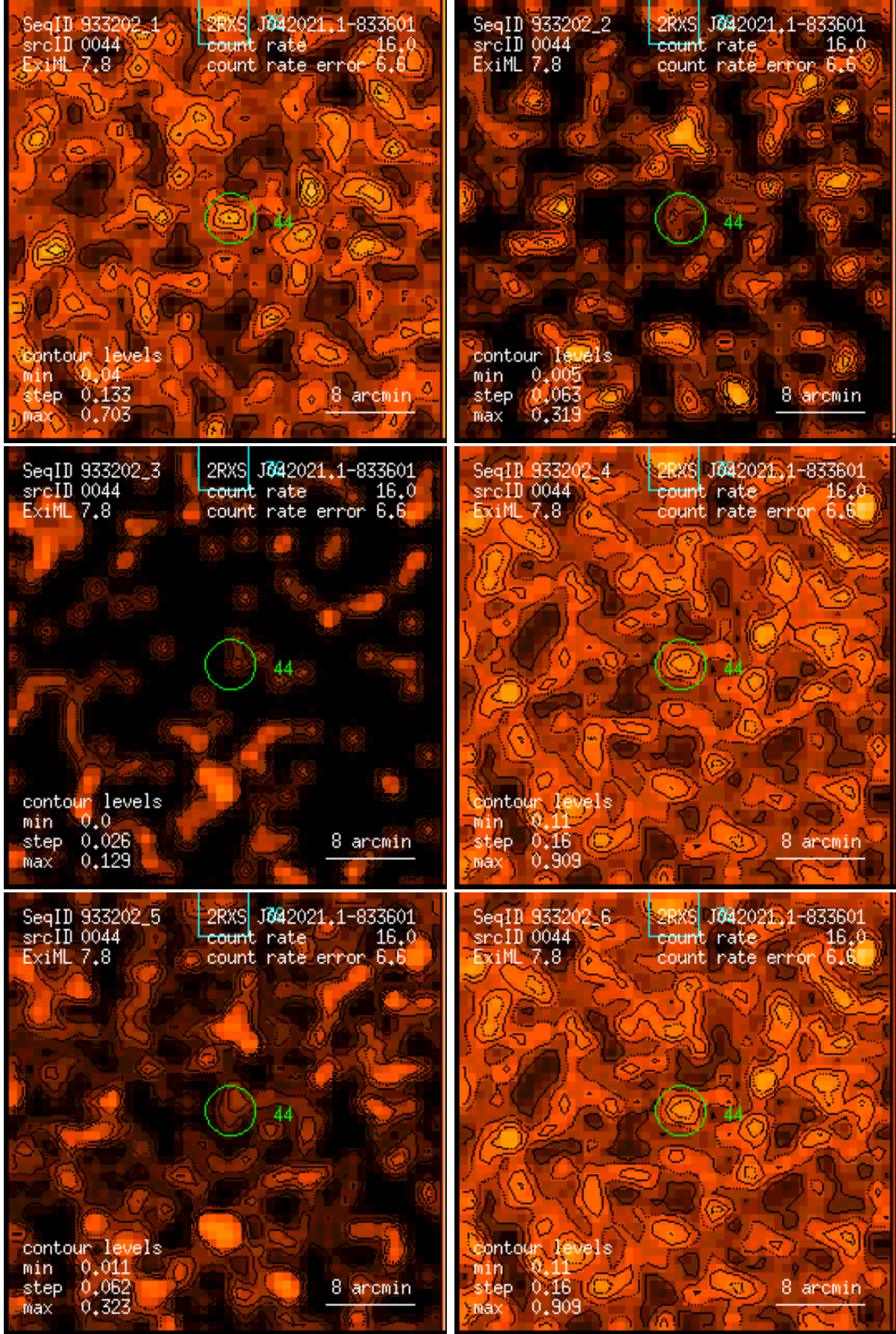
Figure 44: RASS 933202: detection 0044: band rate images, Gaussian filter: (1) PSPC channels 11 – 41, (2) 52 – 90, (3) 91 – 201, (4) 11 – 235, (5) 52 – 201, (6) 11 – 201. Broad band rates in counts/ks. Band rate contour levels in counts/ks/arcmin 2 .
