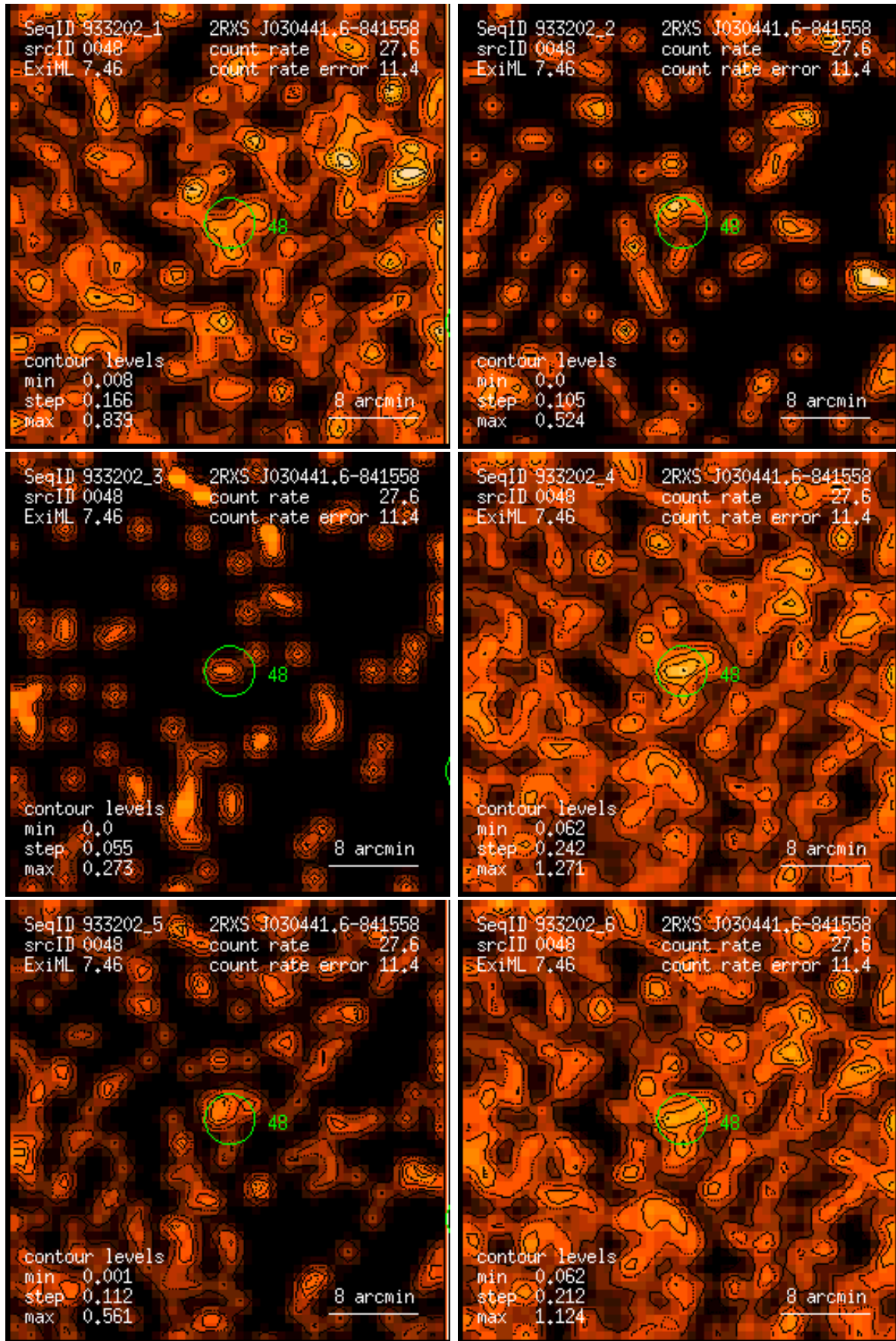
Figure 48: RASS 933202: detection 0048: band rate images, Gaussian filter: (1) PSPC channels 11 – 41, (2) 52 – 90, (3) 91 – 201, (4) 11 – 235, (5) 52 – 201, (6) 11 – 201. Broad band rates in counts/ks. Band rate contour levels in counts/ks/arcmin 2 .
