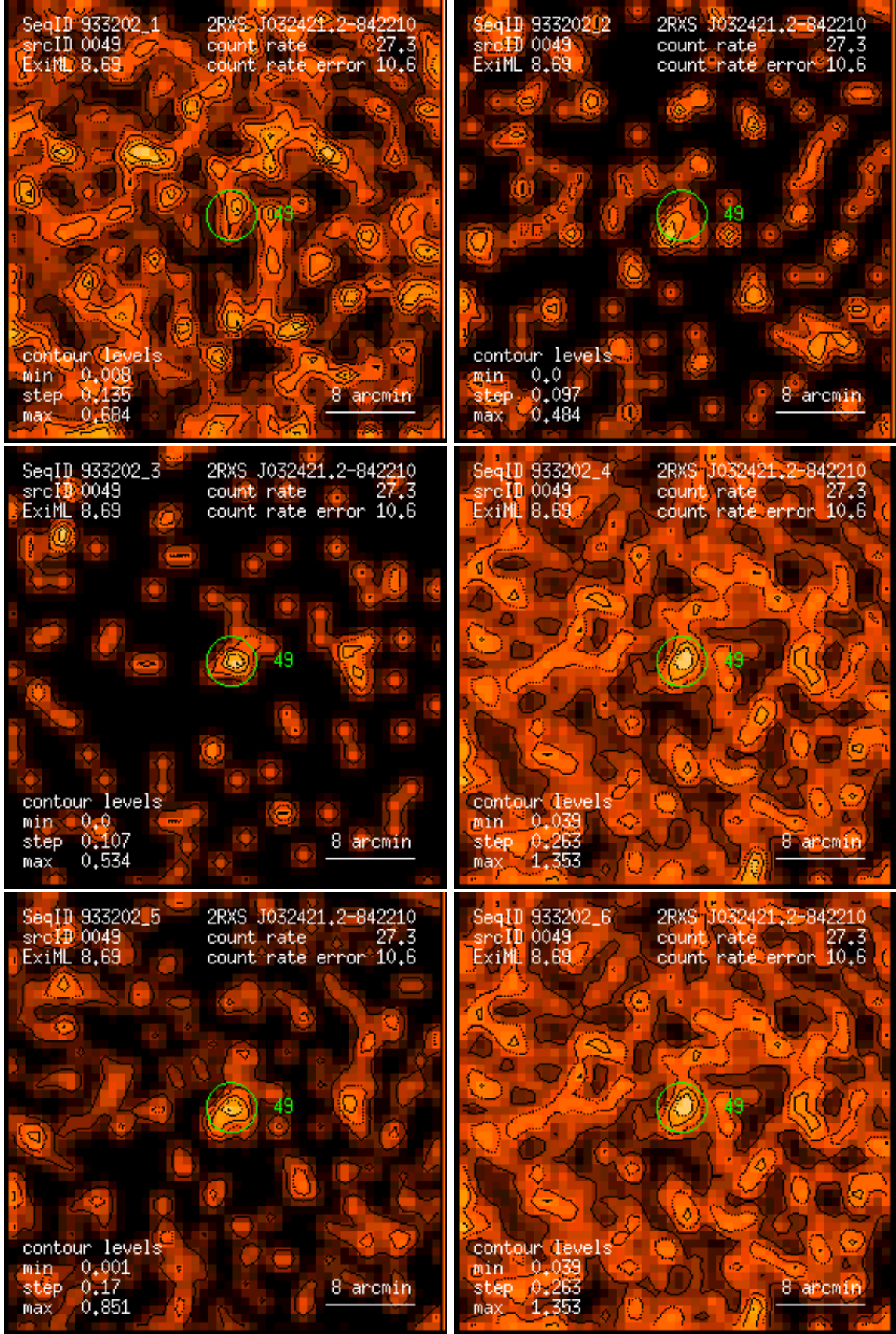
Figure 49: RASS 933202: detection 0049: band rate images, Gaussian filter: (1) PSPC channels 11 – 41, (2) 52 – 90, (3) 91 – 201, (4) 11 – 235, (5) 52 – 201, (6) 11 – 201. Broad band rates in counts/ks. Band rate contour levels in counts/ks/arcmin 2 .
