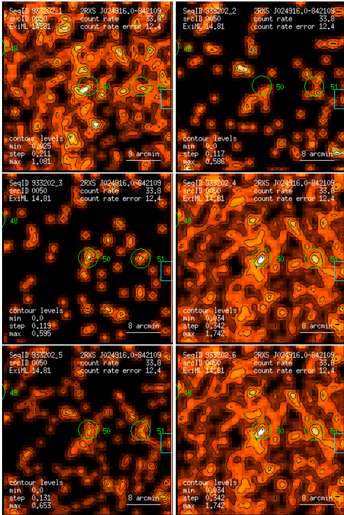
Figure 50: RASS 933202: detection 0050: band rate images, Gaussian filter: (1) PSPC channels 11 – 41, (2) 52 – 90, (3) 91 – 201, (4) 11 – 235, (5) 52 – 201, (6) 11 – 201. Broad band rates in counts/ks. Band rate contour levels in counts/ks/arcmin 2 .
