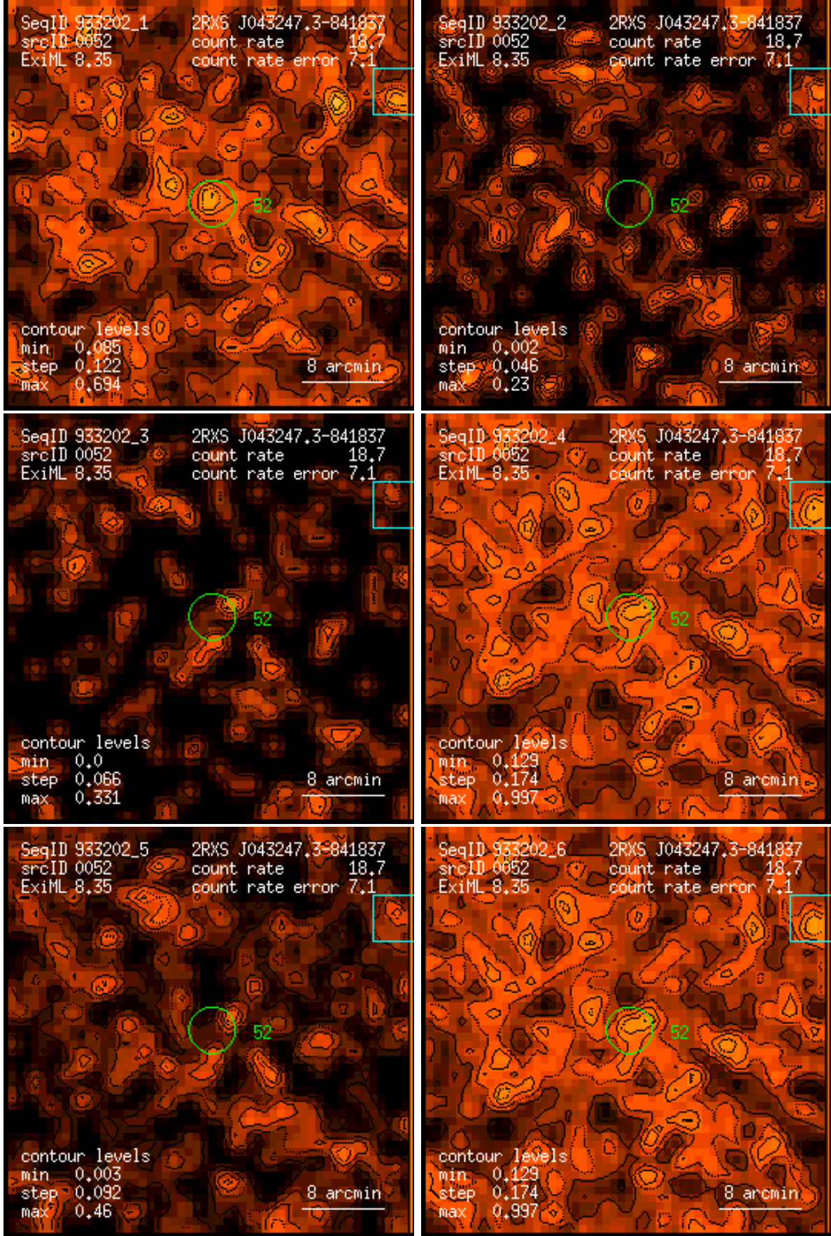
Figure 52: RASS 933202: detection 0052: band rate images, Gaussian filter: (1) PSPC channels 11 – 41, (2) 52 – 90, (3) 91 – 201, (4) 11 – 235, (5) 52 – 201, (6) 11 – 201. Broad band rates in counts/ks. Band rate contour levels in counts/ks/arcmin 2 .
