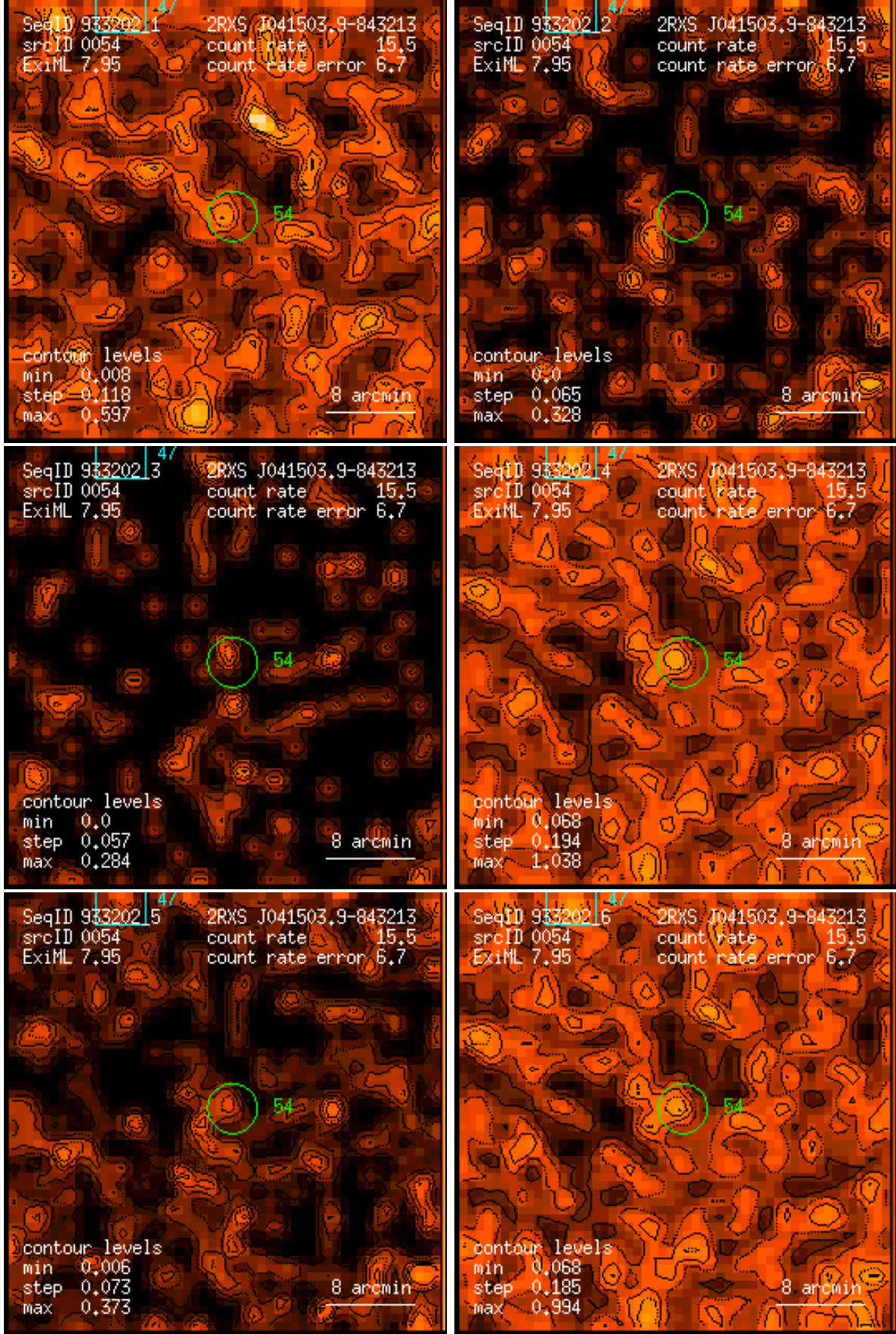
Figure 54: RASS 933202: detection 0054: band rate images, Gaussian filter: (1) PSPC channels 11 – 41, (2) 52 – 90, (3) 91 – 201, (4) 11 – 235, (5) 52 – 201, (6) 11 – 201. Broad band rates in counts/ks. Band rate contour levels in counts/ks/arcmin 2 .
