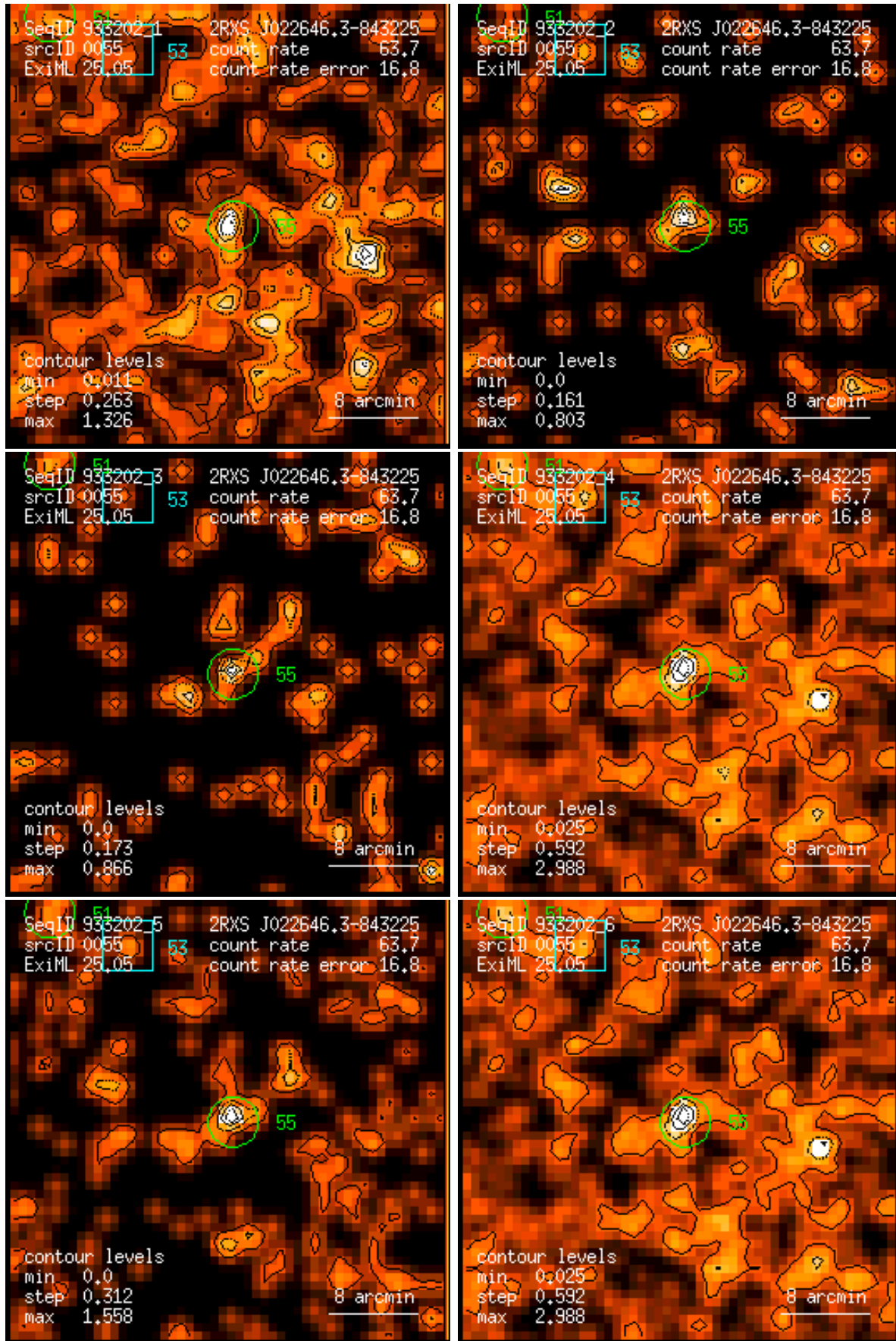
Figure 55: RASS 933202: detection 0055: band rate images, Gaussian filter: (1) PSPC channels 11 – 41, (2) 52 – 90, (3) 91 – 201, (4) 11 – 235, (5) 52 – 201, (6) 11 – 201. Broad band rates in counts/ks. Band rate contour levels in counts/ks/arcmin 2 .
