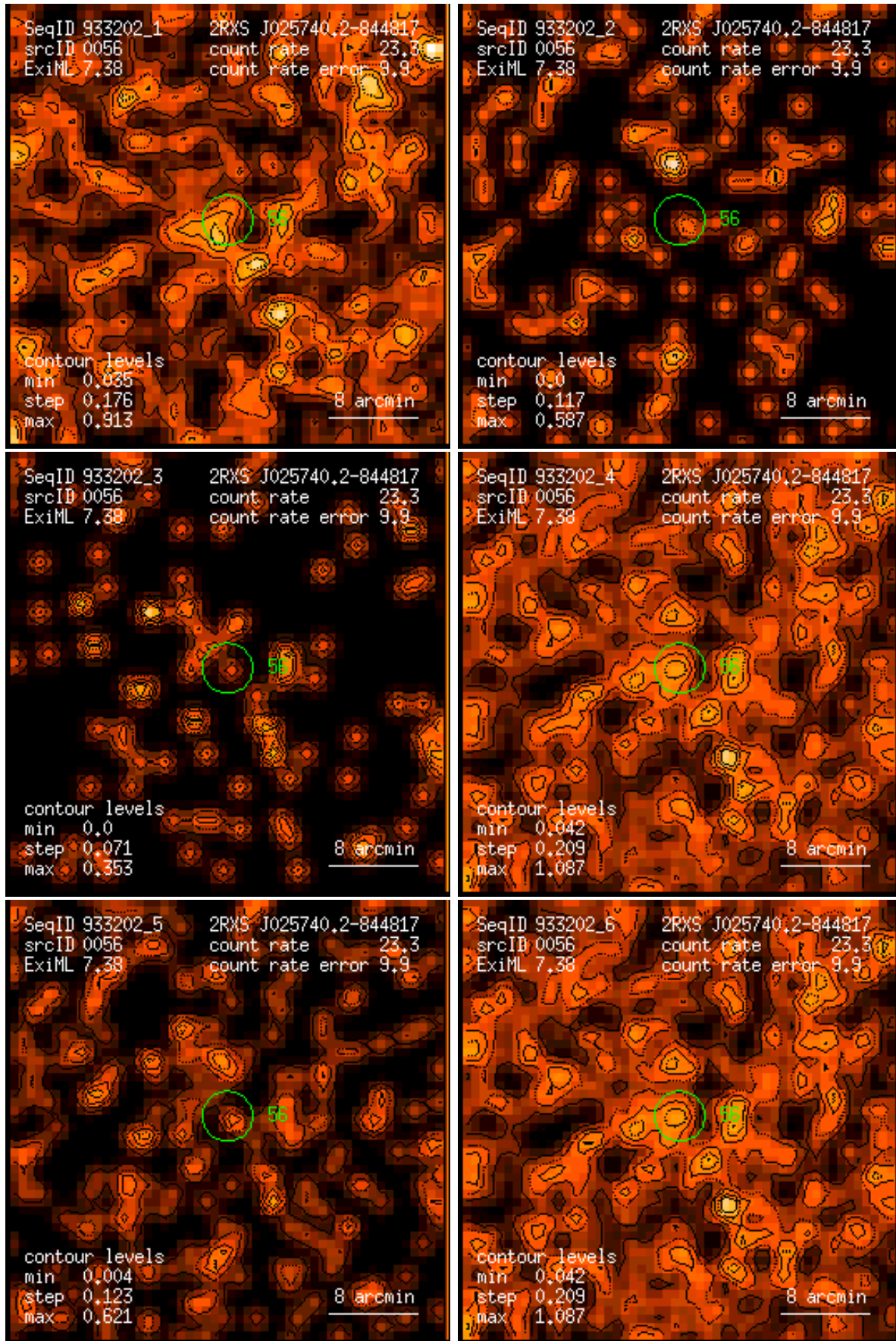
Figure 56: RASS 933202: detection 0056: band rate images, Gaussian filter: (1) PSPC channels 11 – 41, (2) 52 – 90, (3) 91 – 201, (4) 11 – 235, (5) 52 – 201, (6) 11 – 201. Broad band rates in counts/ks. Band rate contour levels in counts/ks/arcmin 2 .
