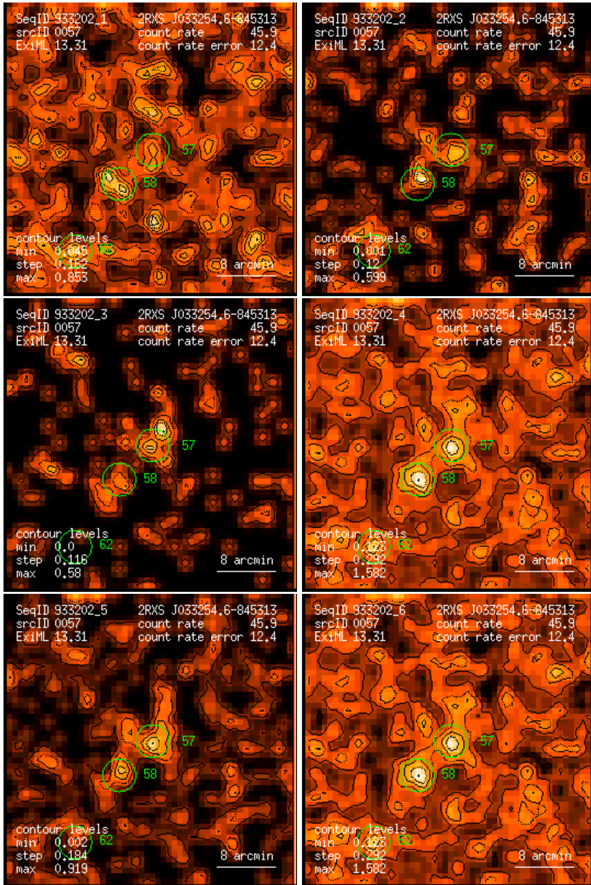
Figure 57: RASS 933202: detection 0057: band rate images, Gaussian filter: (1) PSPC channels 11 – 41, (2) 52 – 90, (3) 91 – 201, (4) 11 – 235, (5) 52 – 201, (6) 11 – 201. Broad band rates in counts/ks. Band rate contour levels in counts/ks/arcmin 2 .
