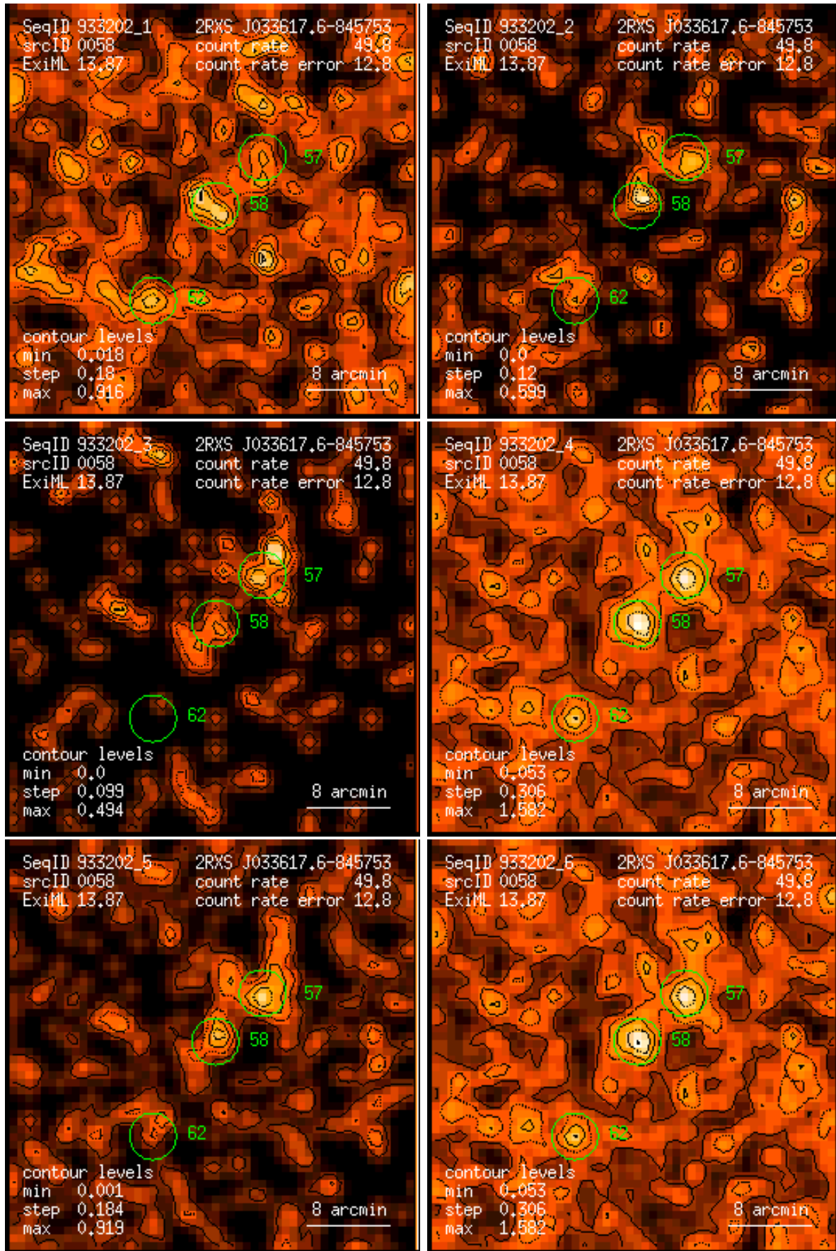
Figure 58: RASS 933202: detection 0058: band rate images, Gaussian filter: (1) PSPC channels 11 – 41, (2) 52 – 90, (3) 91 – 201, (4) 11 – 235, (5) 52 – 201, (6) 11 – 201. Broad band rates in counts/ks. Band rate contour levels in counts/ks/arcmin 2 .
