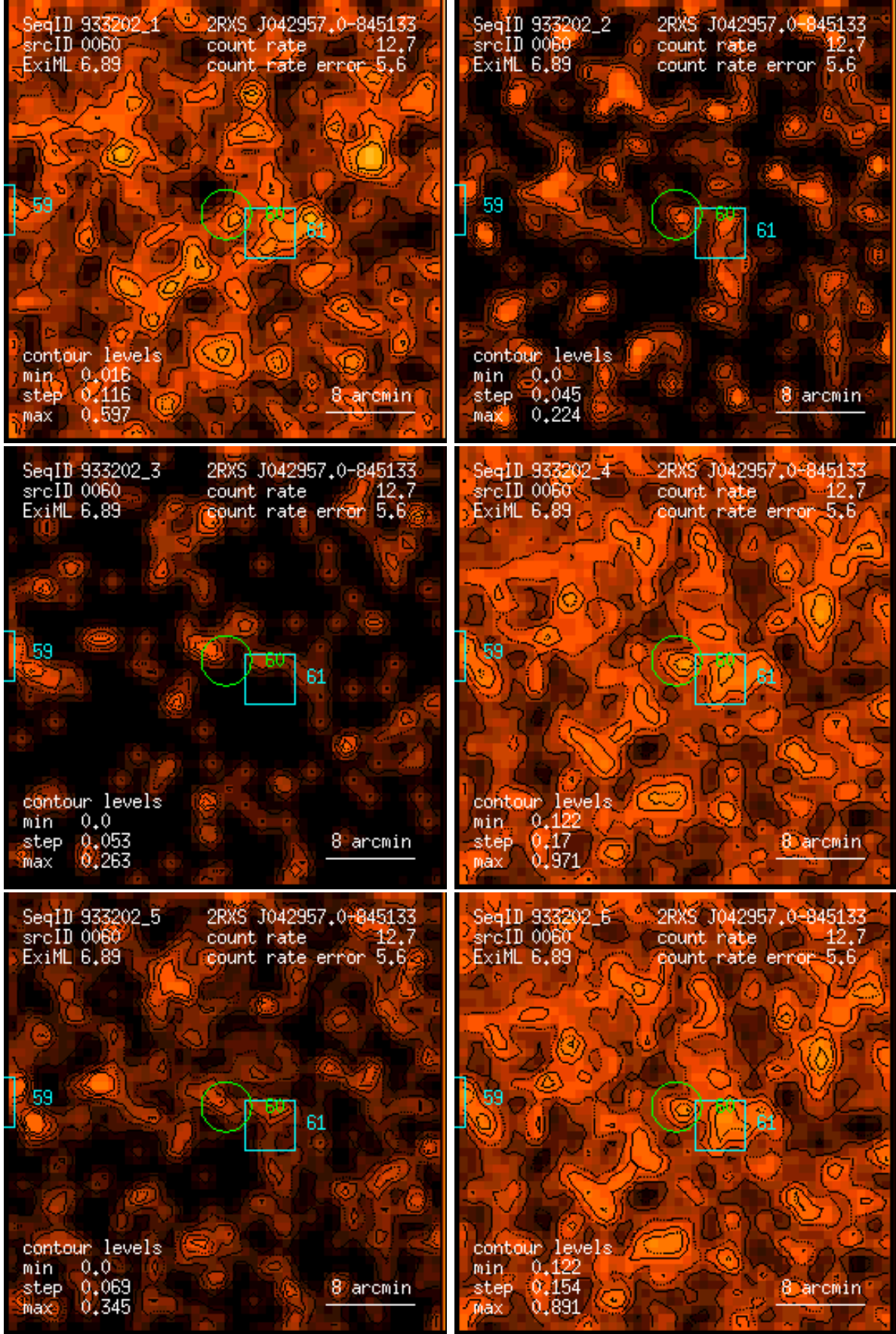
Figure 60: RASS 933202: detection 0060: band rate images, Gaussian filter: (1) PSPC channels 11 – 41, (2) 52 – 90, (3) 91 – 201, (4) 11 – 235, (5) 52 – 201, (6) 11 – 201. Broad band rates in counts/ks. Band rate contour levels in counts/ks/arcmin 2 .
