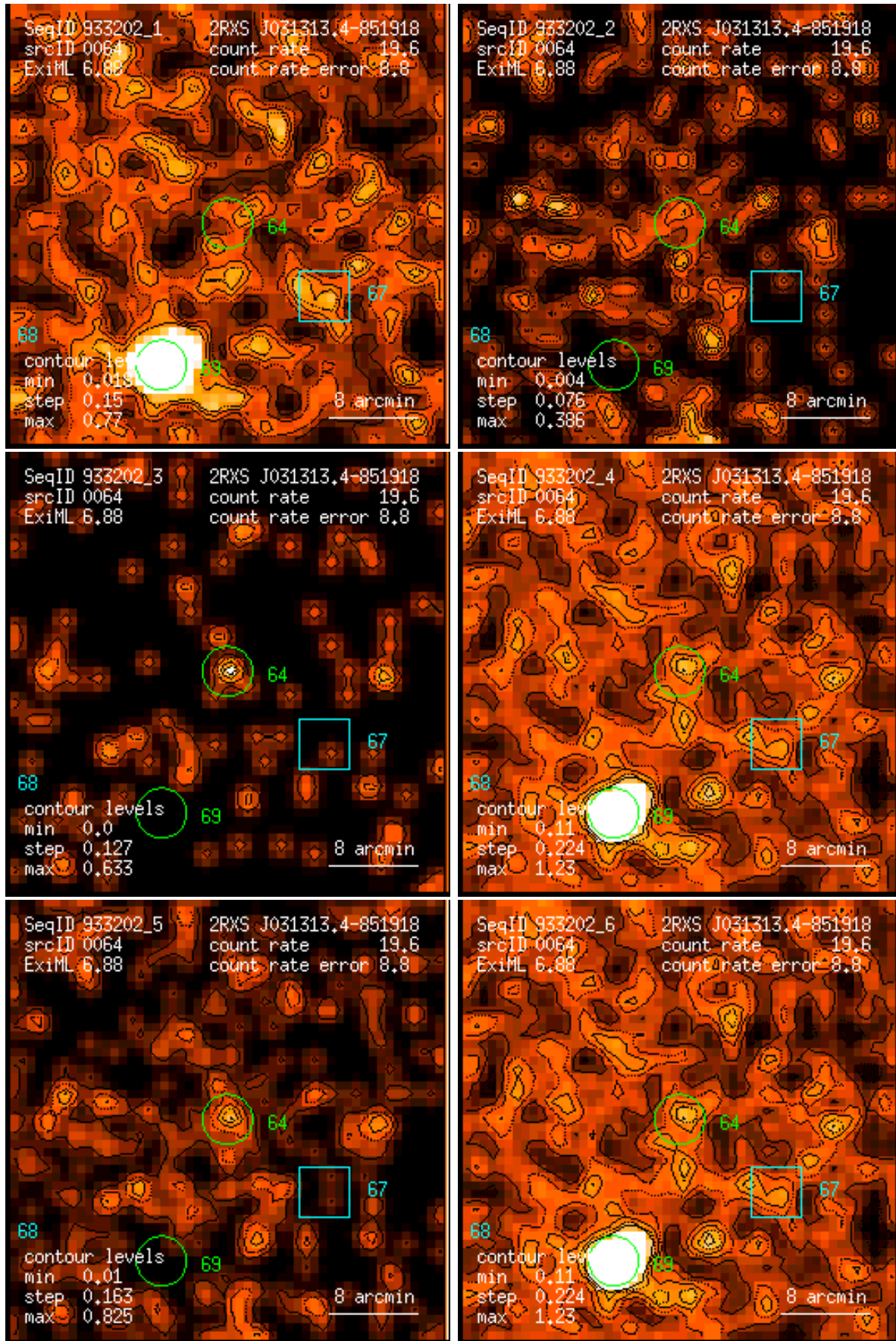
Figure 64: RASS 933202: detection 0064: band rate images, Gaussian filter: (1) PSPC channels 11 – 41, (2) 52 – 90, (3) 91 – 201, (4) 11 – 235, (5) 52 – 201, (6) 11 – 201. Broad band rates in counts/ks. Band rate contour levels in counts/ks/arcmin 2 .
