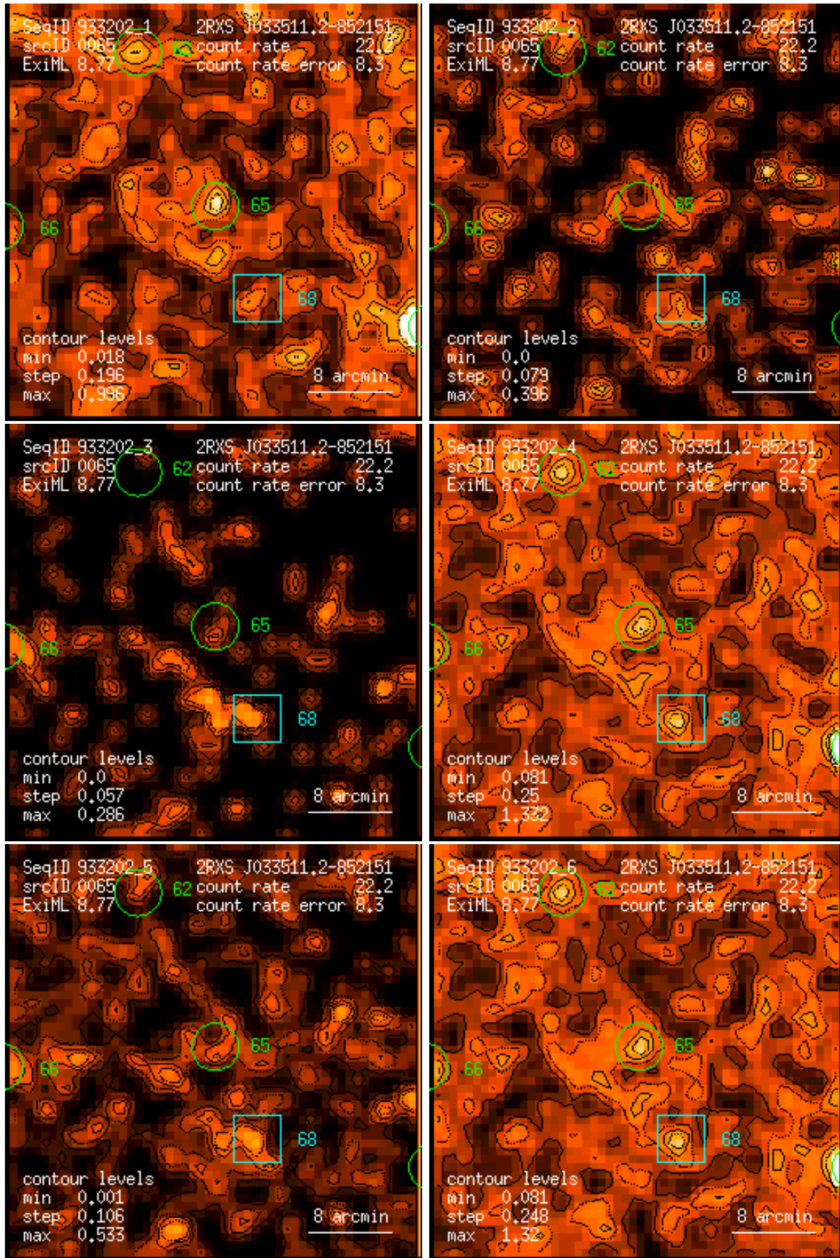
Figure 65: RASS 933202: detection 0065: band rate images, Gaussian filter: (1) PSPC channels 11 – 41, (2) 52 – 90, (3) 91 – 201, (4) 11 – 235, (5) 52 – 201, (6) 11 – 201. Broad band rates in counts/ks. Band rate contour levels in counts/ks/arcmin 2 .
