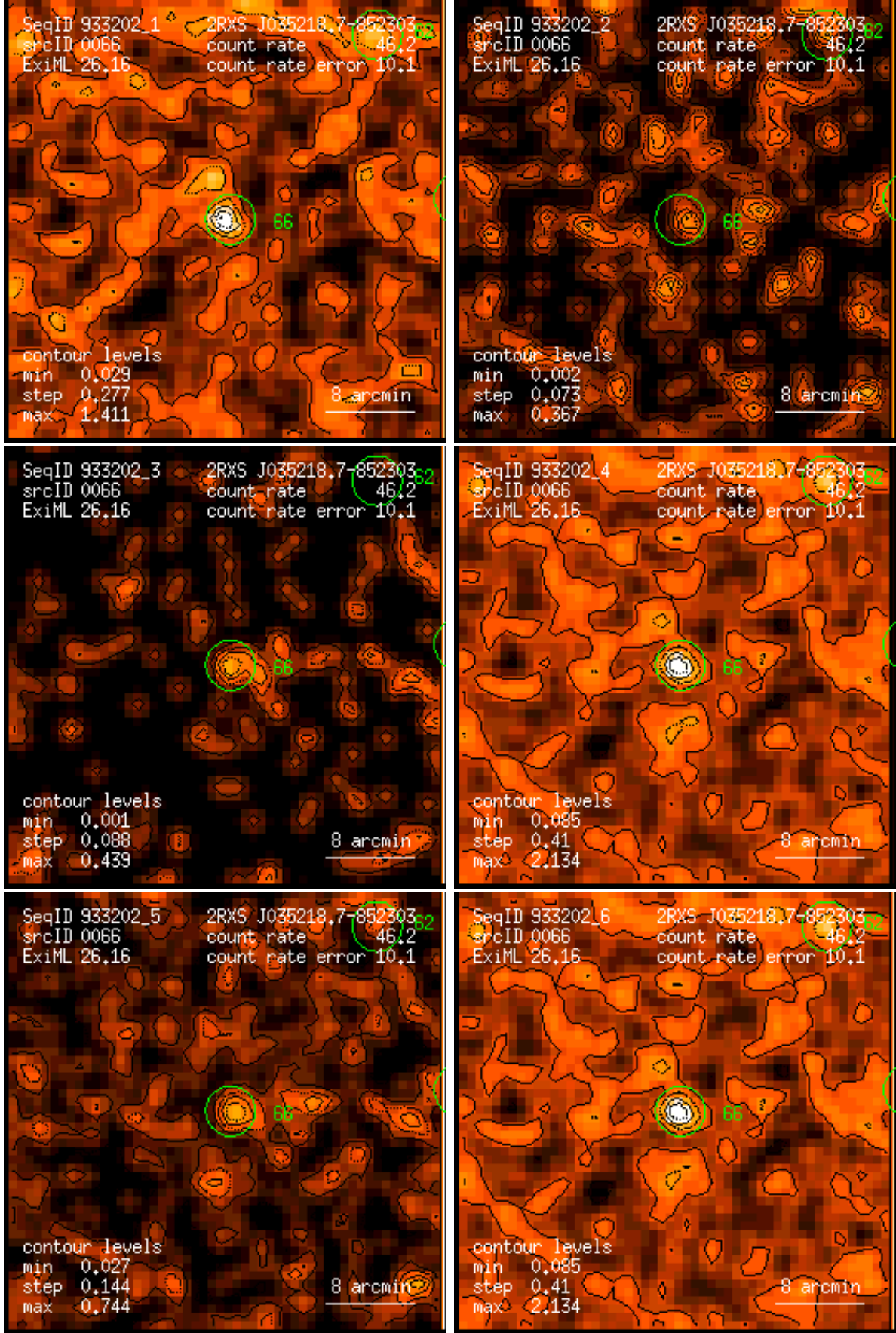
Figure 66: RASS 933202: detection 0066: band rate images, Gaussian filter: (1) PSPC channels 11 – 41, (2) 52 – 90, (3) 91 – 201, (4) 11 – 235, (5) 52 – 201, (6) 11 – 201. Broad band rates in counts/ks. Band rate contour levels in counts/ks/arcmin 2 .
