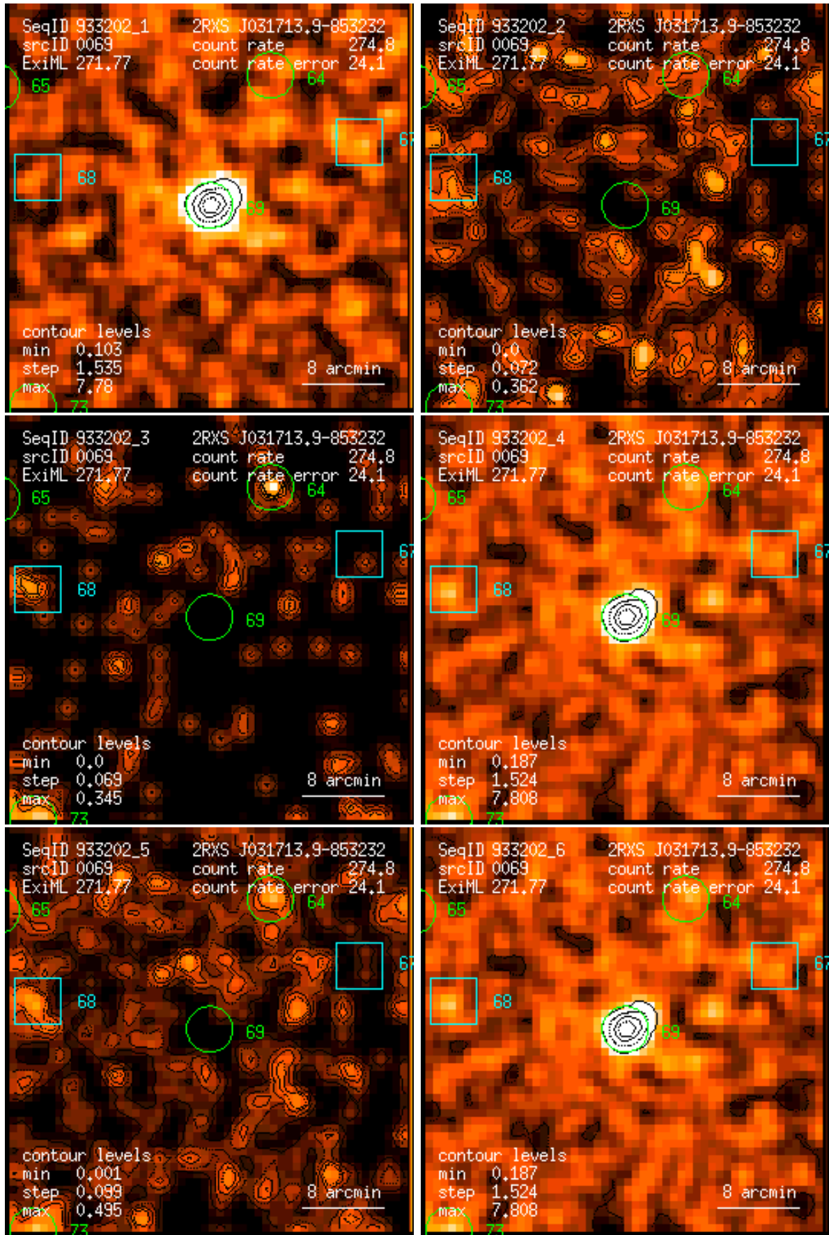
Figure 69: RASS 933202: detection 0069: band rate images, Gaussian filter: (1) PSPC channels 11 – 41, (2) 52 – 90, (3) 91 – 201, (4) 11 – 235, (5) 52 – 201, (6) 11 – 201. Broad band rates in counts/ks. Band rate contour levels in counts/ks/arcmin 2 .
