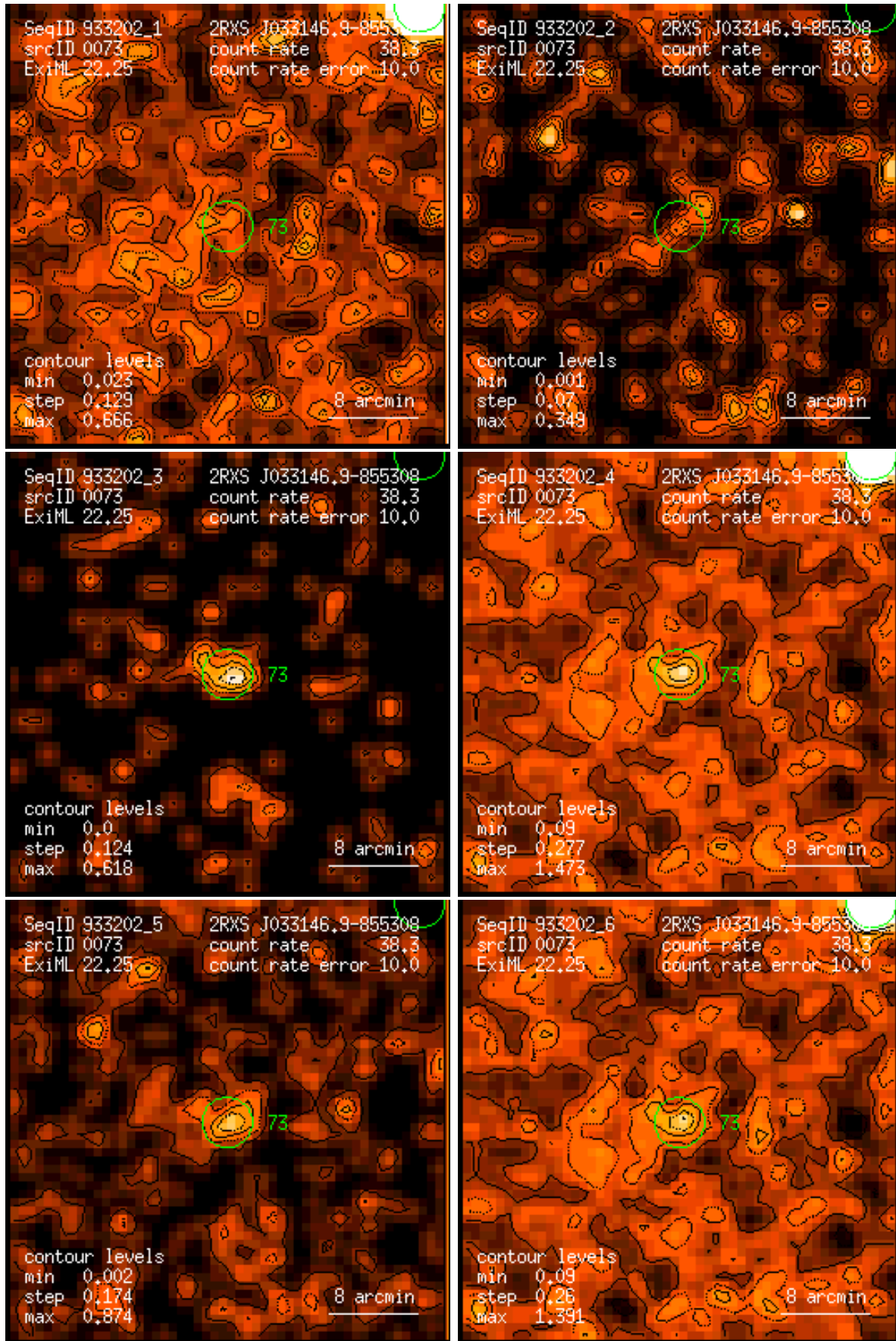
Figure 73: RASS 933202: detection 0073: band rate images, Gaussian filter: (1) PSPC channels 11 – 41, (2) 52 – 90, (3) 91 – 201, (4) 11 – 235, (5) 52 – 201, (6) 11 – 201. Broad band rates in counts/ks. Band rate contour levels in counts/ks/arcmin 2 .
