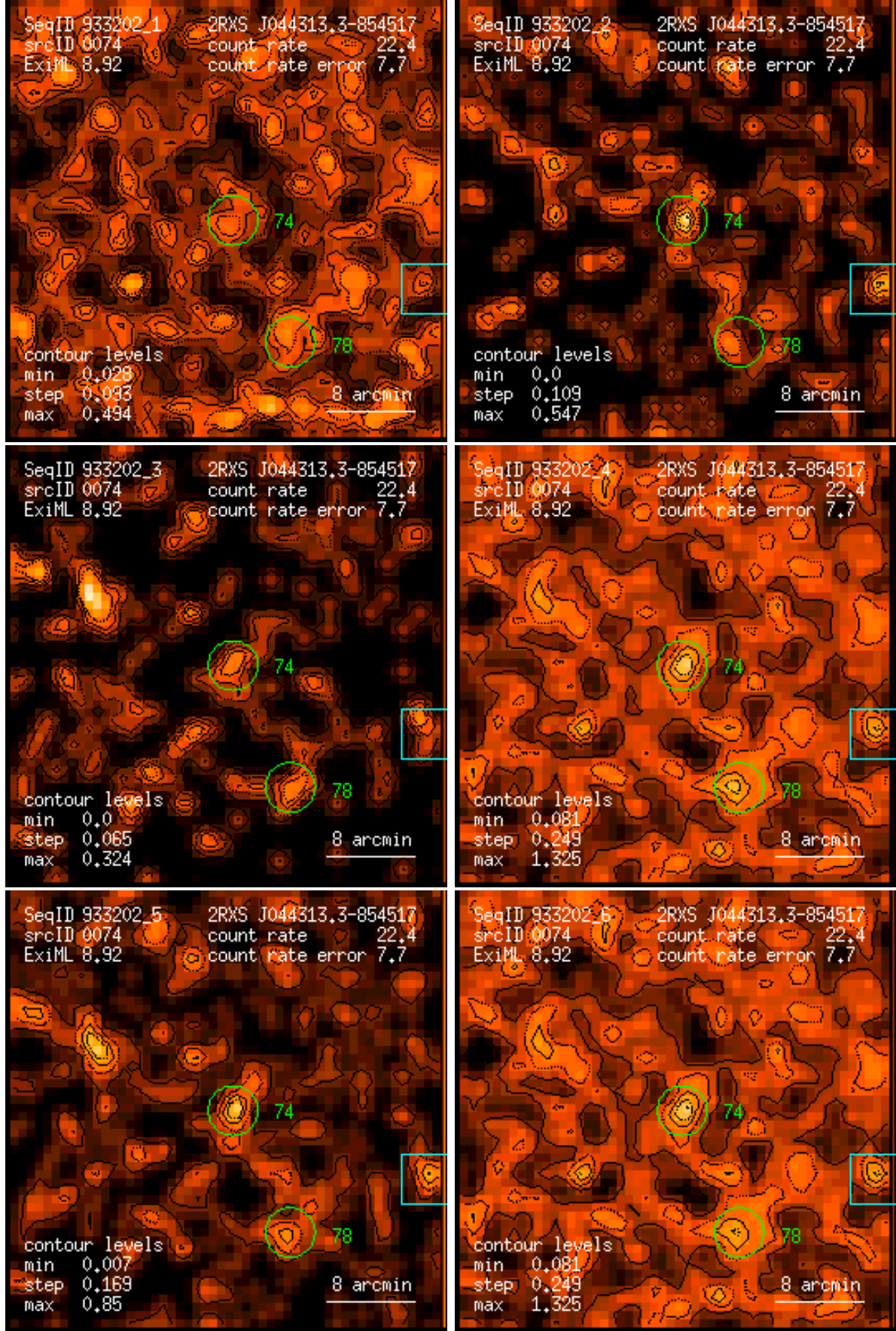
Figure 74: RASS 933202: detection 0074: band rate images, Gaussian filter: (1) PSPC channels 11 – 41, (2) 52 – 90, (3) 91 – 201, (4) 11 – 235, (5) 52 – 201, (6) 11 – 201. Broad band rates in counts/ks. Band rate contour levels in counts/ks/arcmin 2 .
