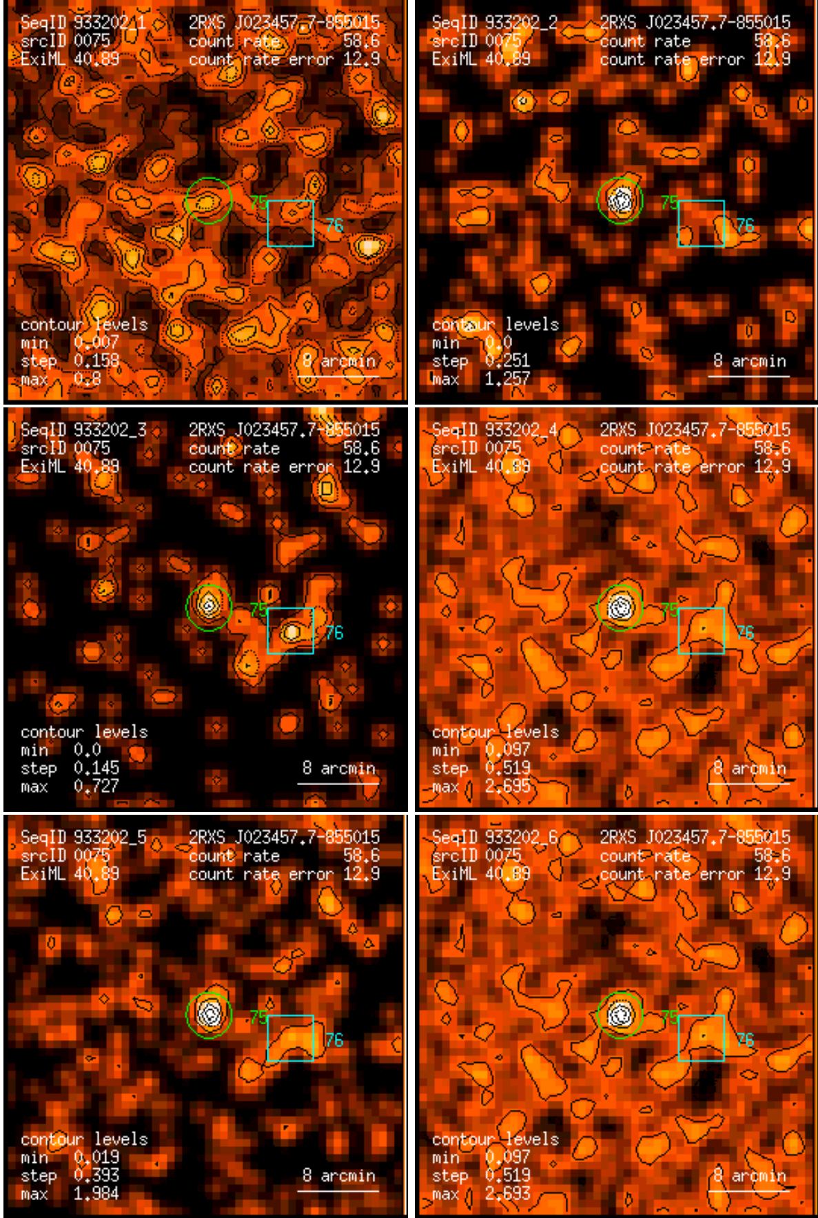
Figure 75: RASS 933202: detection 0075: band rate images, Gaussian filter: (1) PSPC channels 11 – 41, (2) 52 – 90, (3) 91 – 201, (4) 11 – 235, (5) 52 – 201, (6) 11 – 201. Broad band rates in counts/ks. Band rate contour levels in counts/ks/arcmin 2 .
