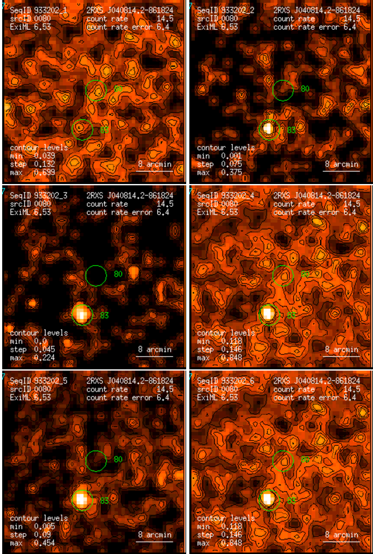
Figure 80: RASS 933202: detection 0080: band rate images, Gaussian filter: (1) PSPC channels 11 – 41, (2) 52 – 90, (3) 91 – 201, (4) 11 – 235, (5) 52 – 201, (6) 11 – 201. Broad band rates in counts/ks. Band rate contour levels in counts/ks/arcmin 2 .
