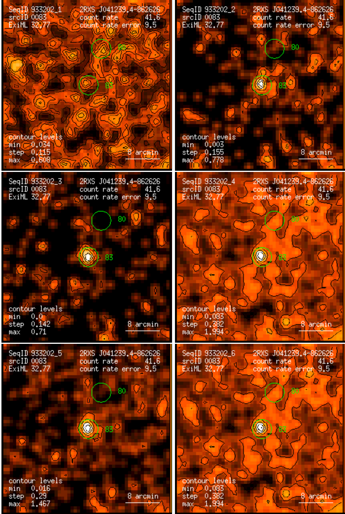
Figure 83: RASS 933202: detection 0083: band rate images, Gaussian filter: (1) PSPC channels 11 – 41, (2) 52 – 90, (3) 91 – 201, (4) 11 – 235, (5) 52 – 201, (6) 11 – 201. Broad band rates in counts/ks. Band rate contour levels in counts/ks/arcmin 2 .
