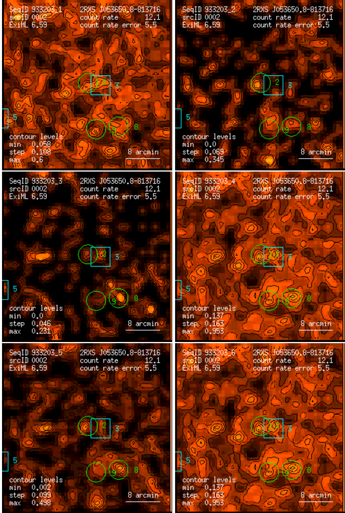
Figure 2: RASS 933203: detection 0002: band rate images, Gaussian filter: (1) PSPC channels 11 – 41, (2) 52 – 90, (3) 91 – 201, (4) 11 – 235, (5) 52 – 201, (6) 11 – 201. Broad band rates in counts/ks. Band rate contour levels in counts/ks/arcmin 2 .
