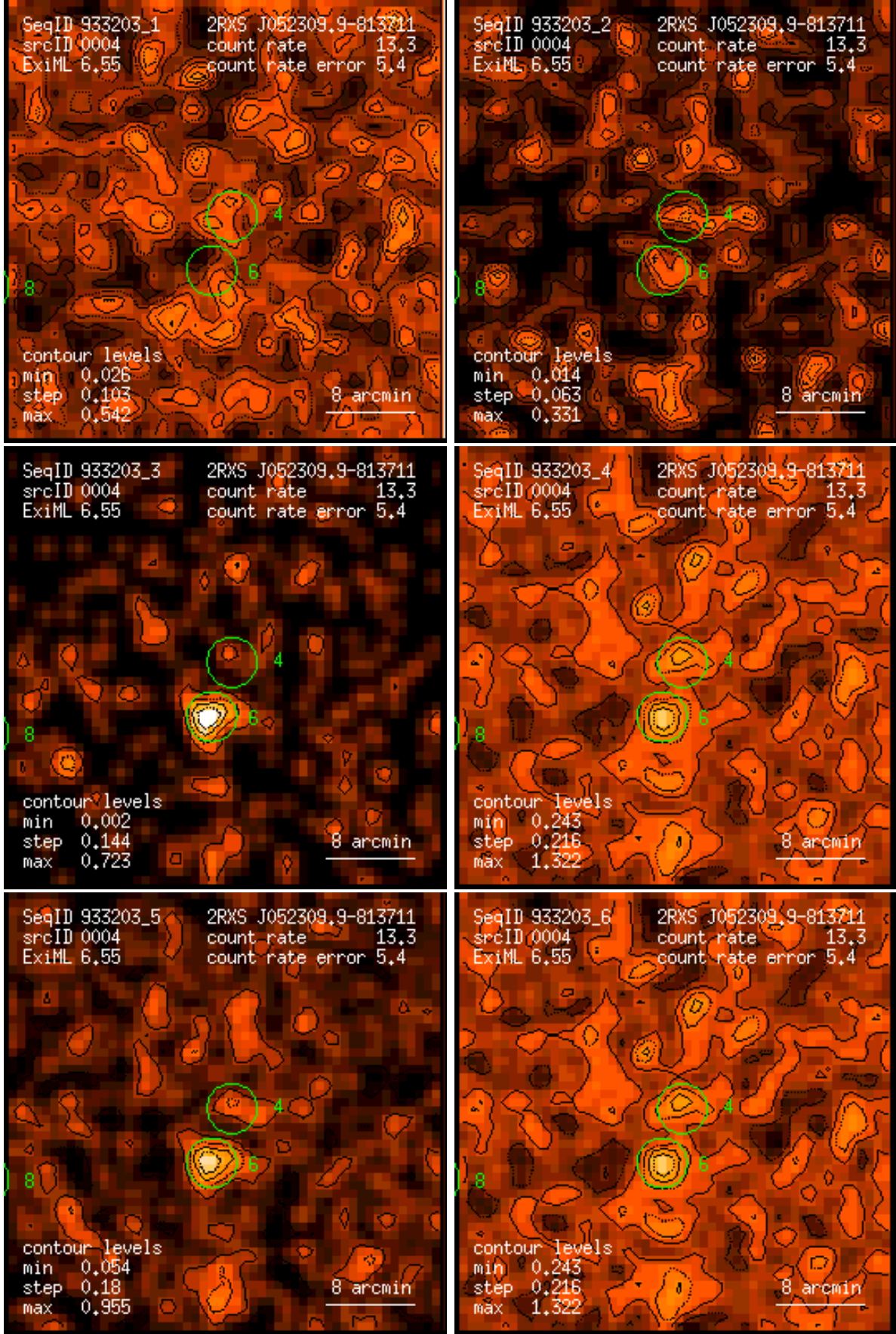
Figure 4: RASS 933203: detection 0004: band rate images, Gaussian filter: (1) PSPC channels 11 – 41, (2) 52 – 90, (3) 91 – 201, (4) 11 – 235, (5) 52 – 201, (6) 11 – 201. Broad band rates in counts/ks. Band rate contour levels in counts/ks/arcmin 2 .
