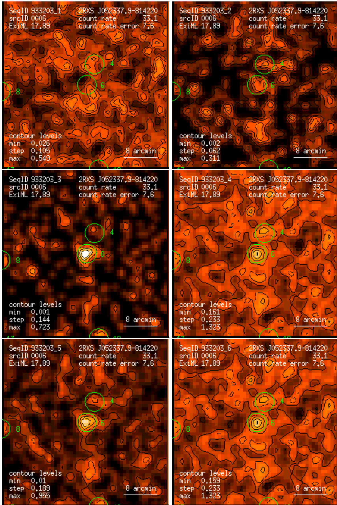
Figure 6: RASS 933203: detection 0006: band rate images, Gaussian filter: (1) PSPC channels 11 – 41, (2) 52 – 90, (3) 91 – 201, (4) 11 – 235, (5) 52 – 201, (6) 11 – 201. Broad band rates in counts/ks. Band rate contour levels in counts/ks/arcmin 2 .
