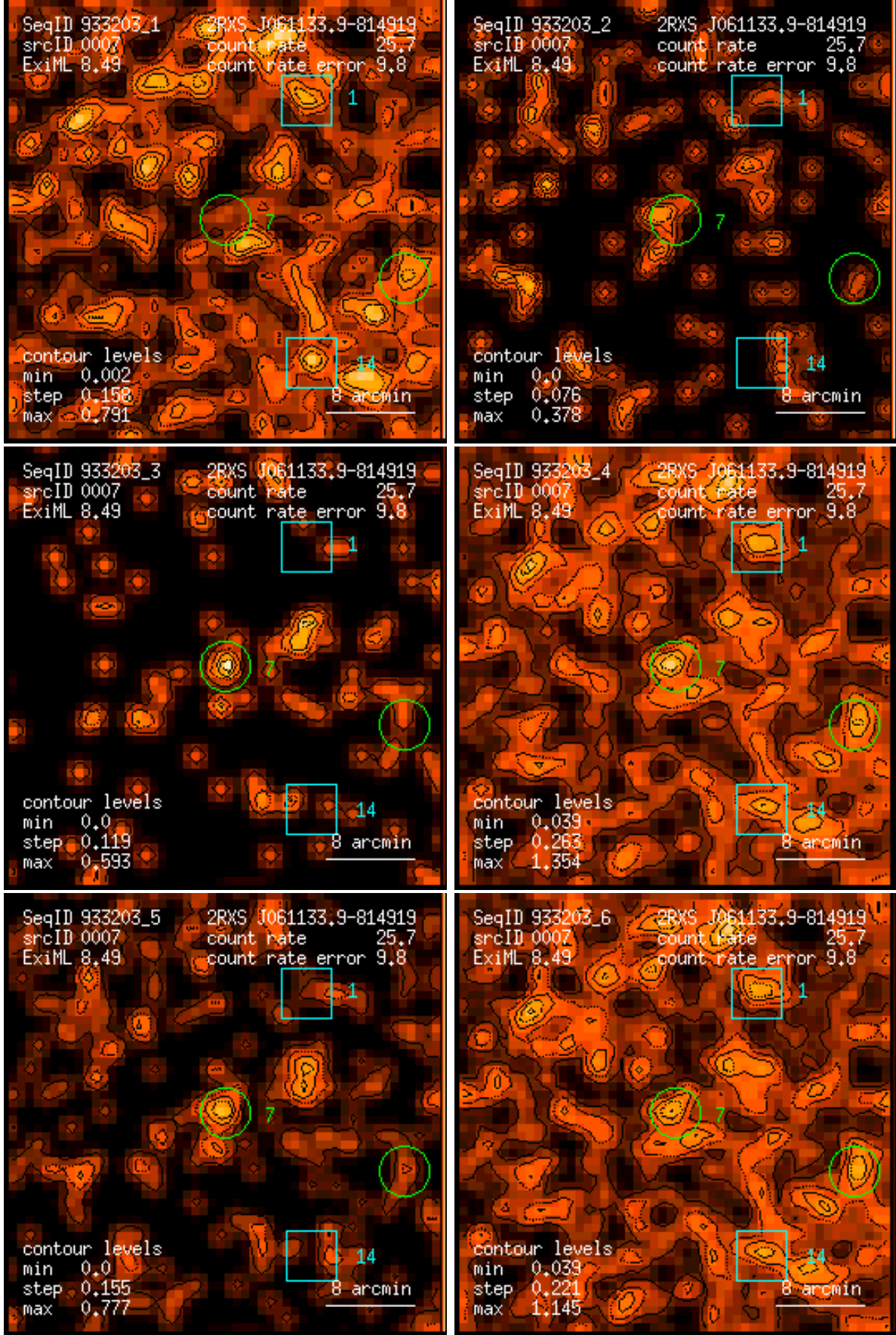
Figure 7: RASS 933203: detection 0007: band rate images, Gaussian filter: (1) PSPC channels 11 – 41, (2) 52 – 90, (3) 91 – 201, (4) 11 – 235, (5) 52 – 201, (6) 11 – 201. Broad band rates in counts/ks. Band rate contour levels in counts/ks/arcmin 2 .
