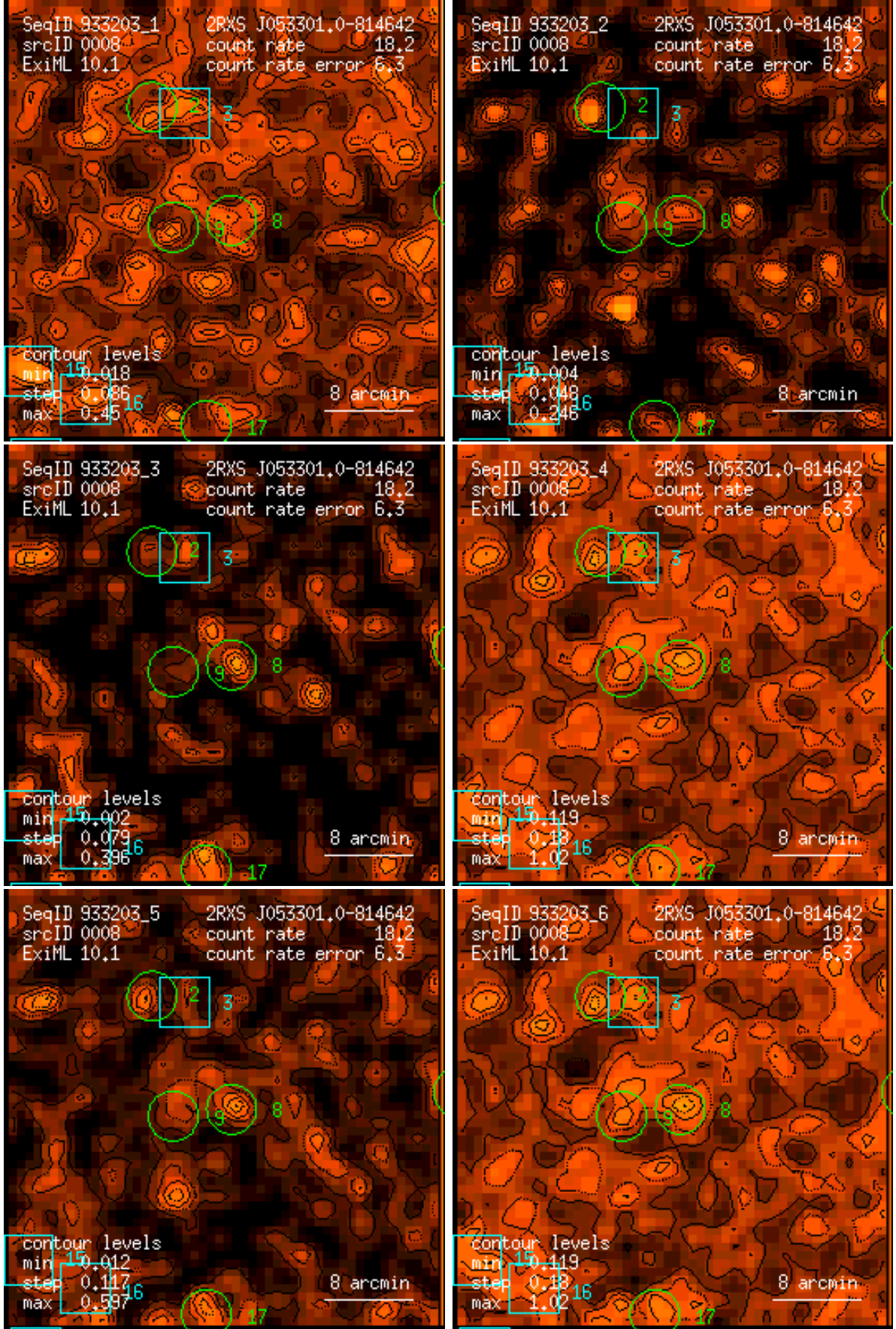
Figure 8: RASS 933203: detection 0008: band rate images, Gaussian filter: (1) PSPC channels 11 – 41, (2) 52 – 90, (3) 91 – 201, (4) 11 – 235, (5) 52 – 201, (6) 11 – 201. Broad band rates in counts/ks. Band rate contour levels in counts/ks/arcmin 2 .
